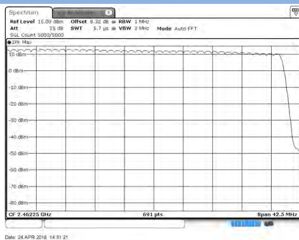
GFSK 2.4415 GHz ~ 2.4835 GHz
