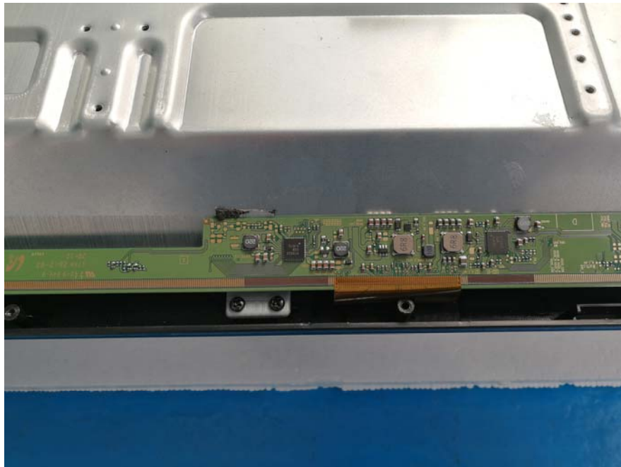
EUT – PCB-3 View-3
