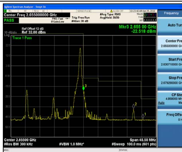
Band41_20MHz_16QAM_41140_1RB#99
