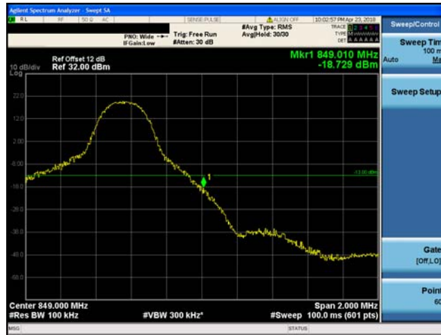
Band5_5MHz_QPSK_20625_1RB#24
