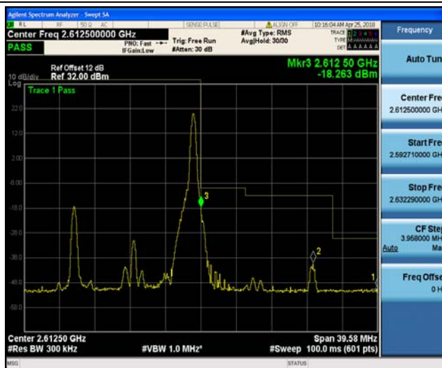
Band41_15MHz_QPSK_40740_1RB#74
