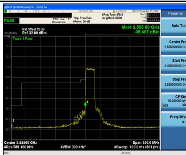
Band41_10MHz_16QAM_40290_50RB#0
