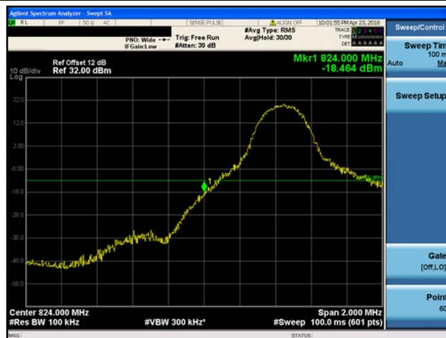
Band5_5MHz_16QAM_20425_1RB#0
