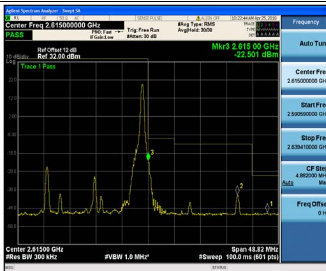
Band41_20MHz_QPSK_40740_1RB#99
