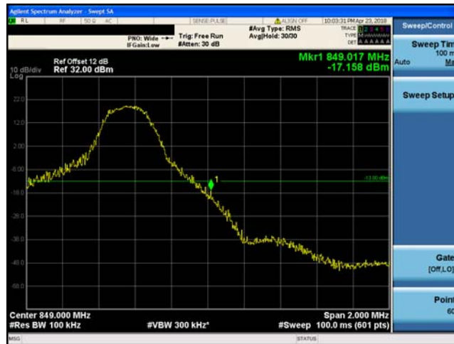
Band5_5MHz_16QAM_20625_1RB#24
