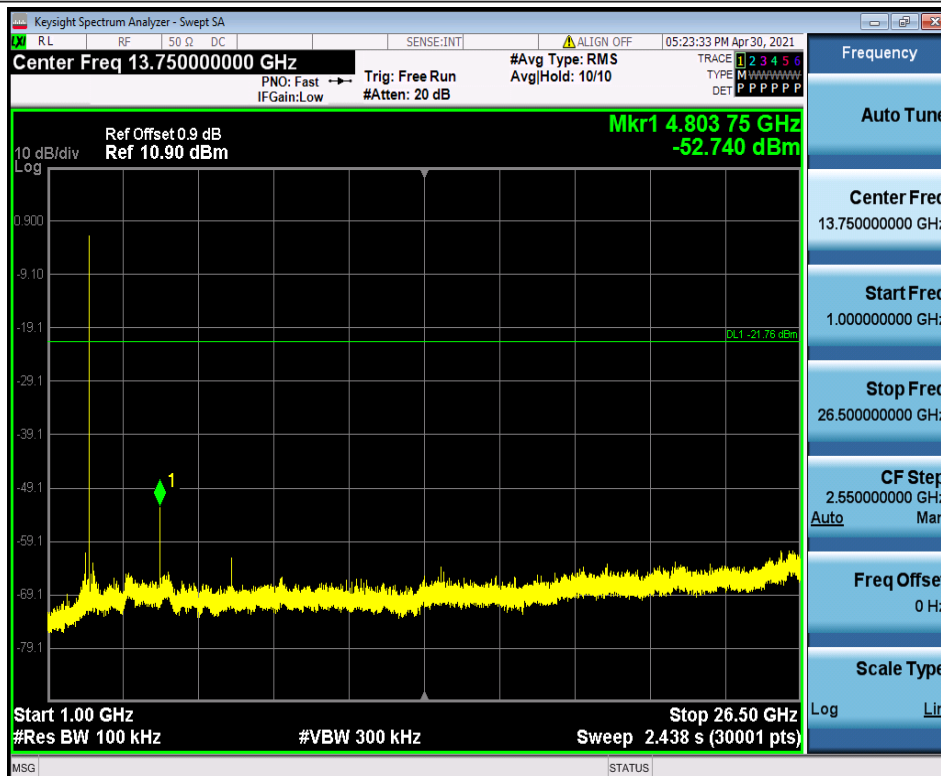
BLE_1M_Ant1_2402_1000~26500
