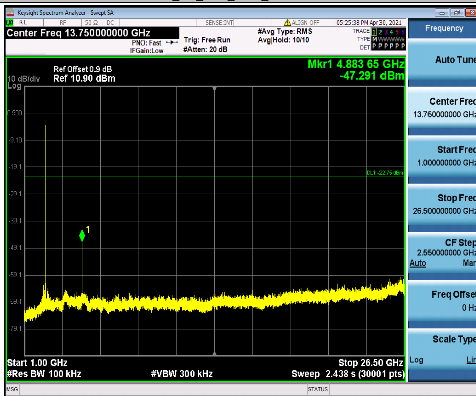
BLE_1M_Ant1_2480_0~Reference
