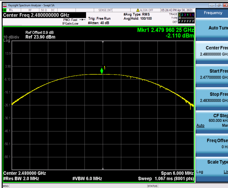
BLE_1M_Ant1_2480
