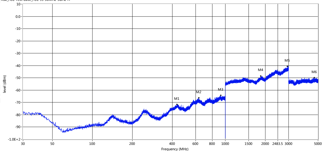
RSE_FCC Test Case_FCC 95 30MHz-5GHz-H
