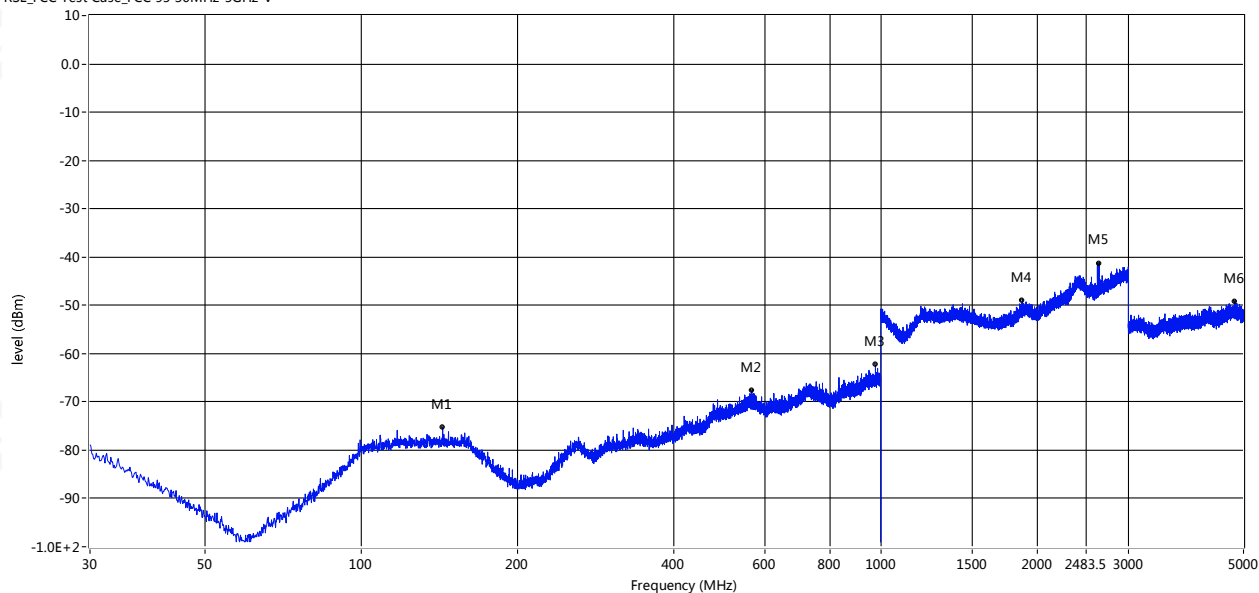
RSE_FCC Test Case_FCC 95 30MHz-5GHz-V
