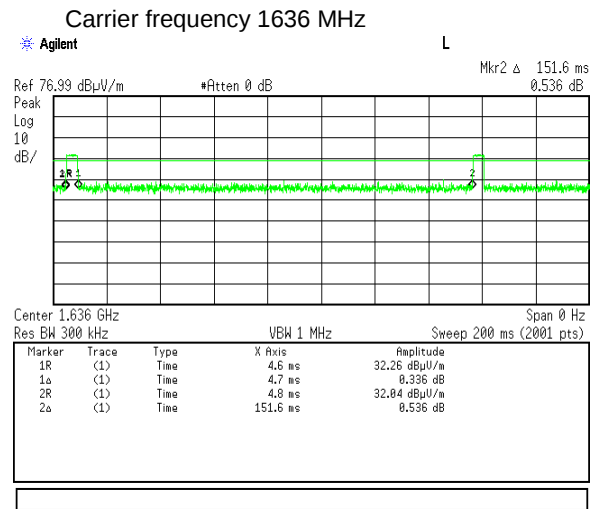
Plot 7.1.36 Number of transmission burst within 100 ms
