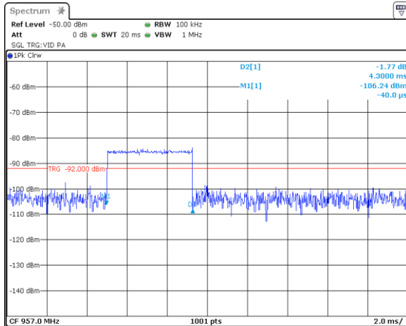
Plot 7.1.34 Transmission burst duration
