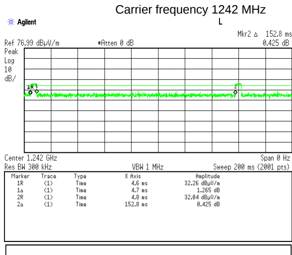
Plot 7.1.36 Number of transmission burst within 100 ms
