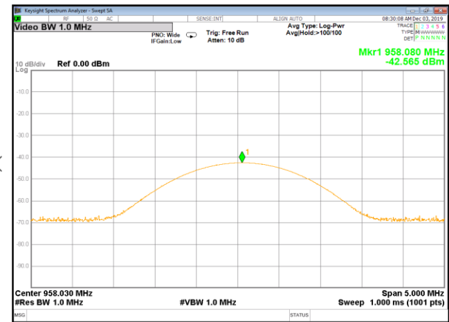
Plot 3.1.2 Power measurements at 958 MHz
