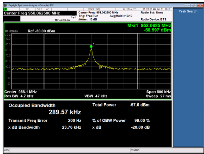
Plot 2 Occupied bandwidth test result at 958 MHz operating frequency
