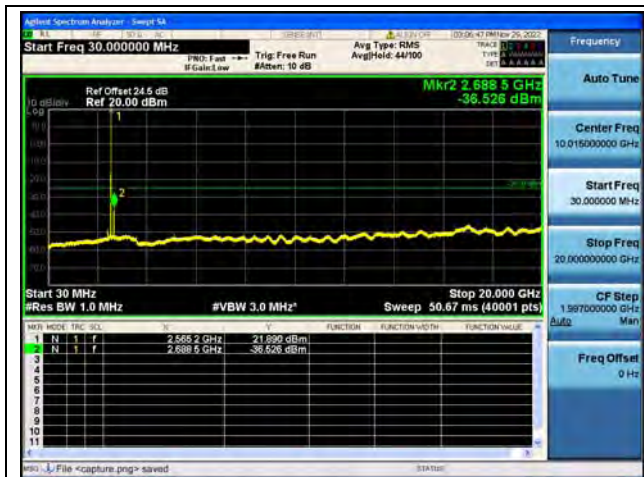
Band7-30M-20G / 5MHz / High CH / QPSK
