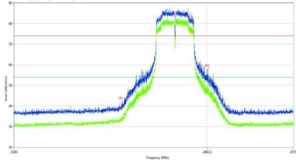
REmission Test case: FCC Part 15C FCC 15.247(E4G) Bandedge 2400
