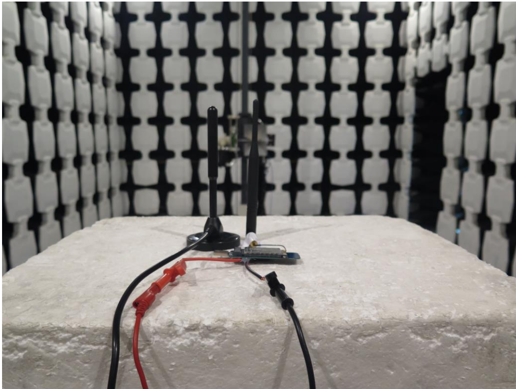
Pic3.Radiated Spurious Emission Test Setup photo (the frequency above 3000MHz)
