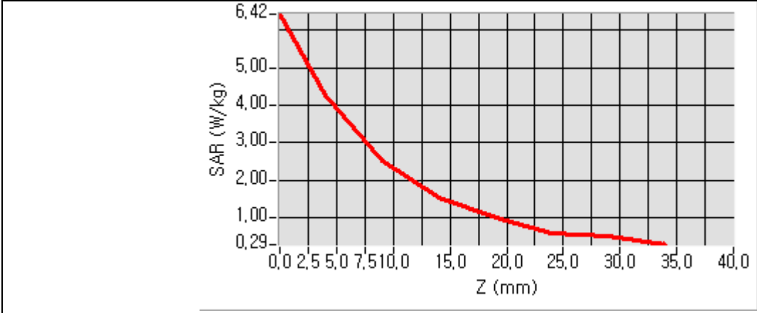
Z Axis Scan (X=0, Y=0)
