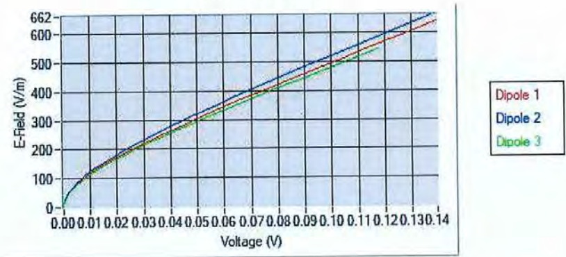
Calibration curves
