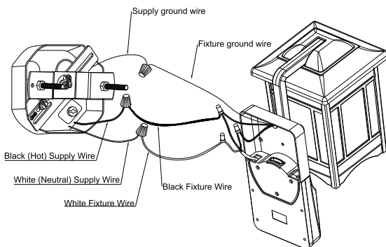
6. Connect the corresponding wires and bare copper wires with a terminal cap. Make sure that the wire cap is screwed
