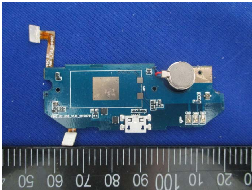
EUT –USB Top View
