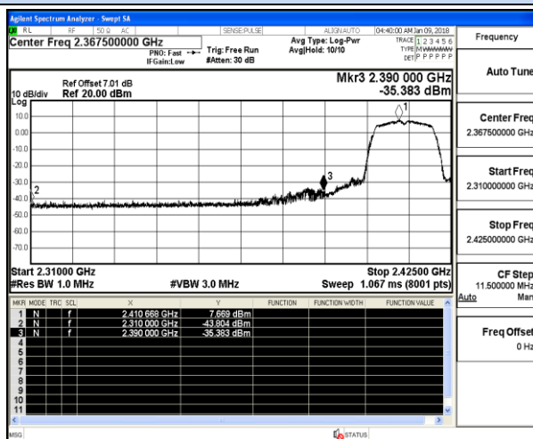
Channel 1 / 2412 MHz – Peak
