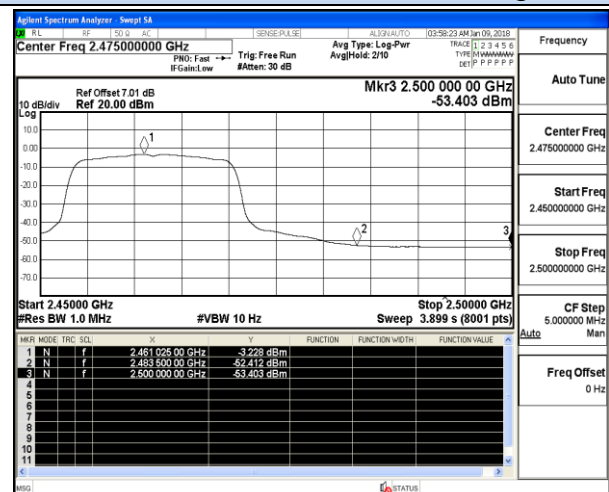
Channel 11 / 2462 MHz – Average
