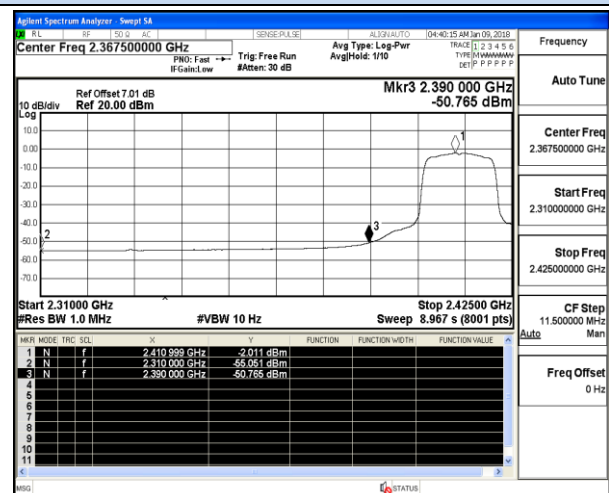
Channel 1 / 2412 MHz – Average
