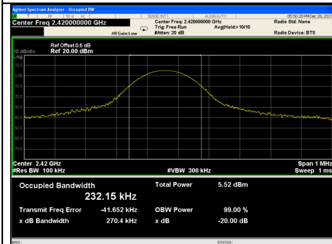
20dB Bandwidth - High CH 2420
