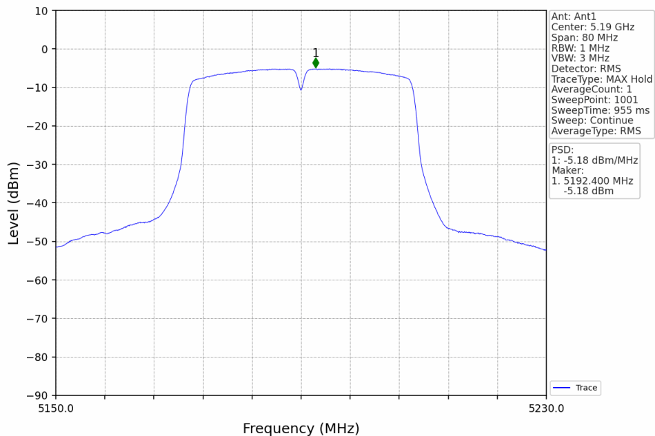
802.11ac(VHT40)_LCH_5190MHz_Ant1_NTNV
