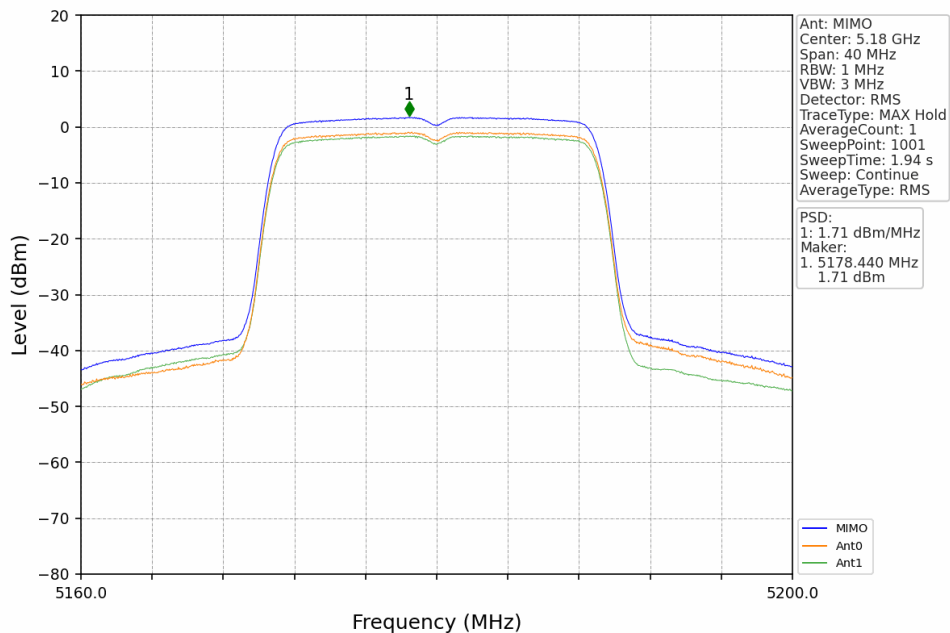
802.11ac(VHT20)_LCH_5180MHz_MIMO_NTNV
