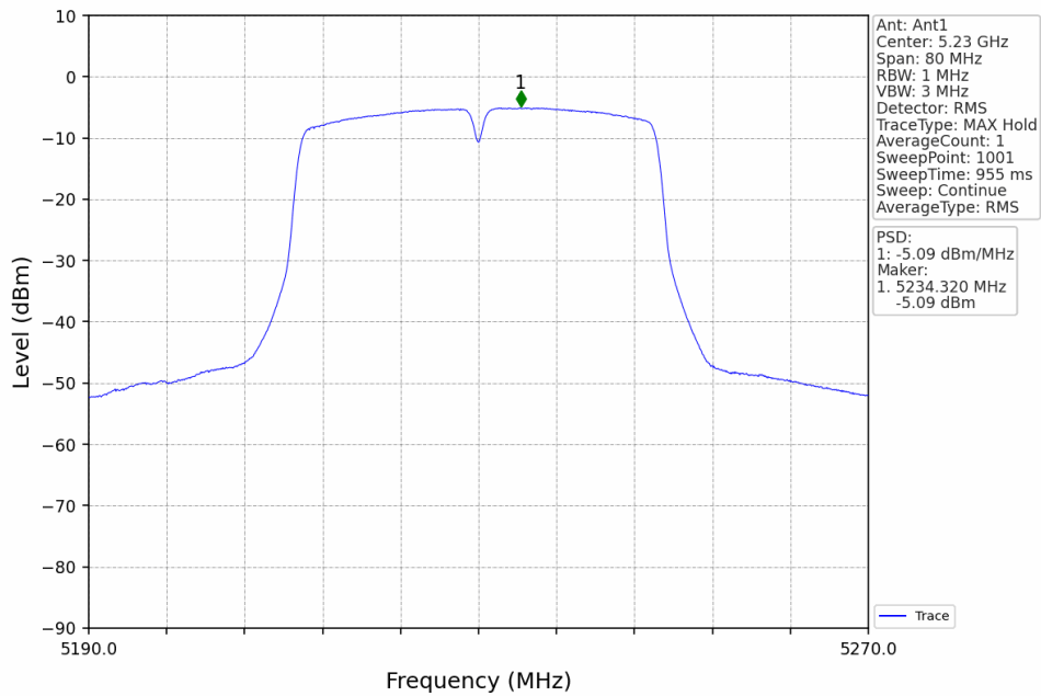
802.11ac(VHT40)_HCH_5230MHz_MIMO_NTNV
