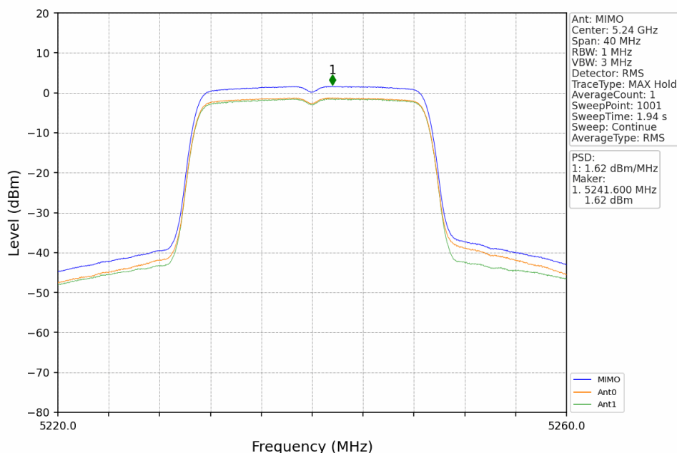
802.11ac(VHT20)_HCH_5240MHz_MIMO_NTNV
