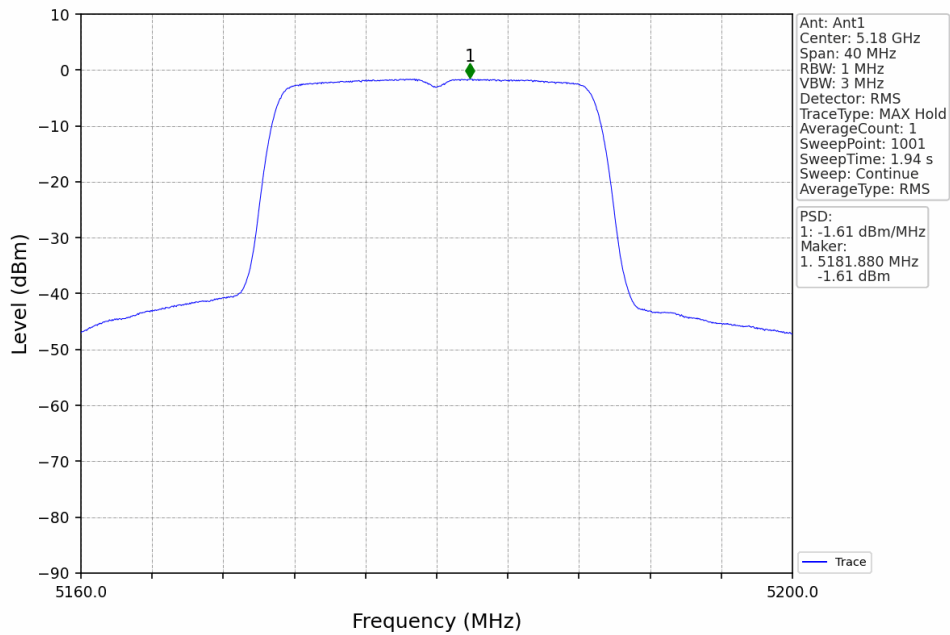
802.11ac(VHT20)_LCH_5180MHz_MIMO_NTNV
