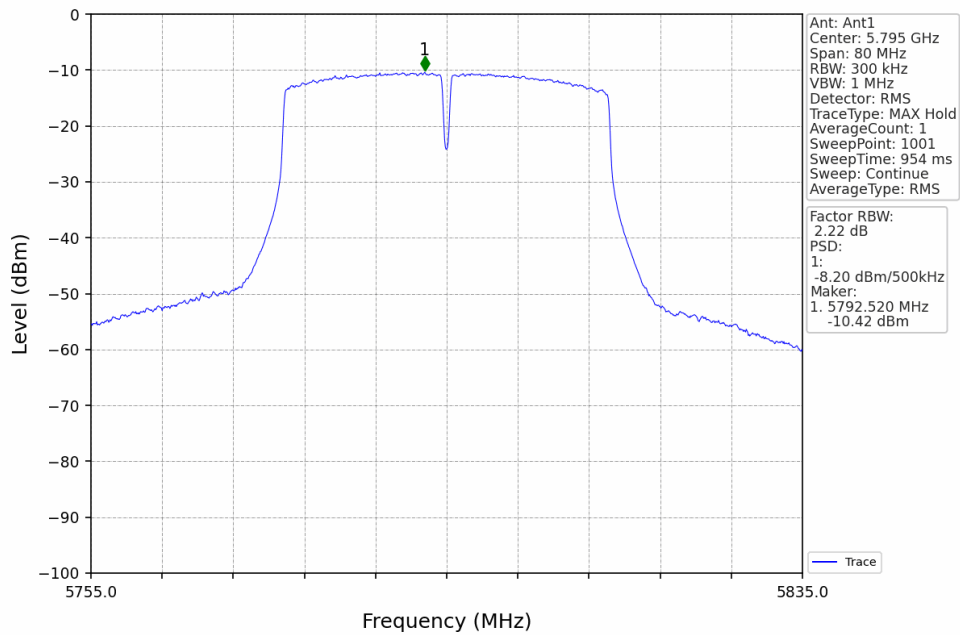
802.11ac(VHT40)_HCH_5795MHz_MIMO_NTNV
