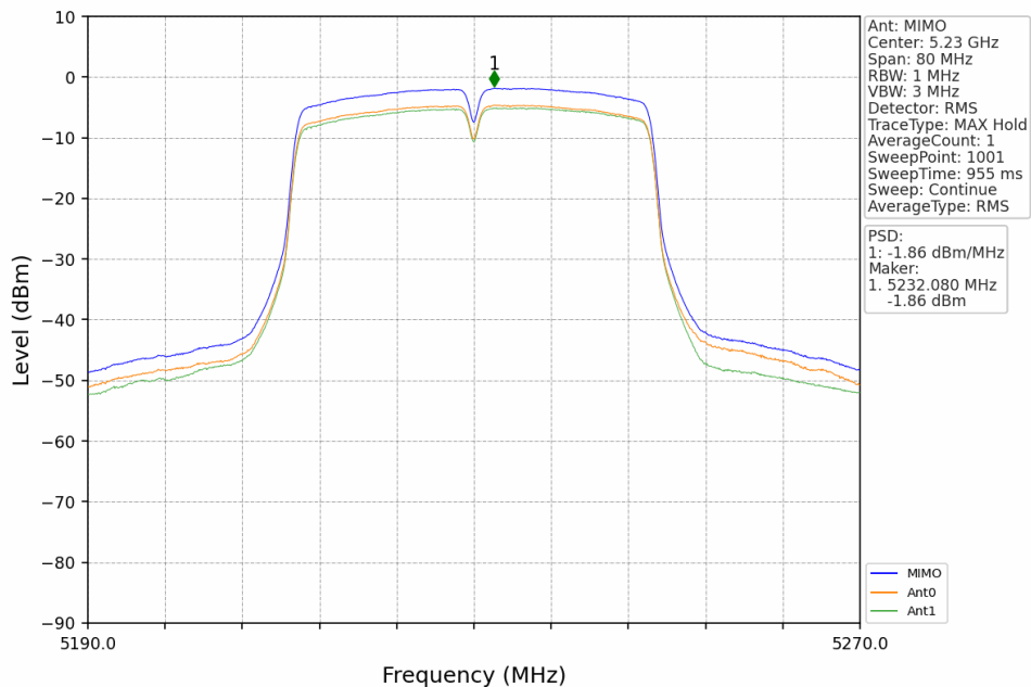
802.11ac(VHT40)_HCH_5230MHz_MIMO_NTNV
