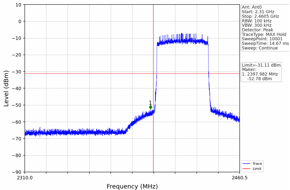
GND_40MHz_LCH_2420.5MHz_Ant0_NTNV
