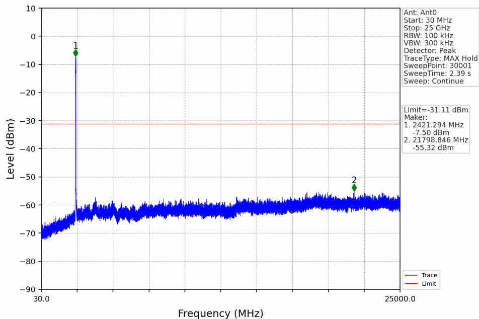
GND_40MHz_LCH_2420.5MHz_Ant0_NTNV
