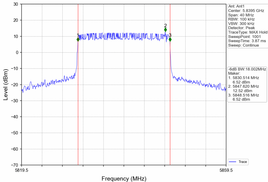
20_HCH_5839.5MHz_Ant1_NTNV
