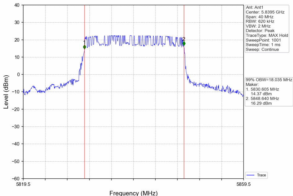
20_HCH_5839.5MHz_Ant1_NTNV
