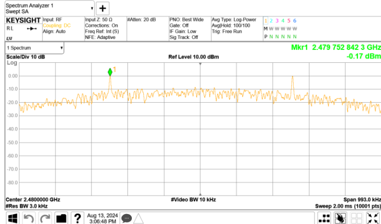
Left, LE 500kbps, Power Spectral Density, Highest Channel (2 480 MHz)
