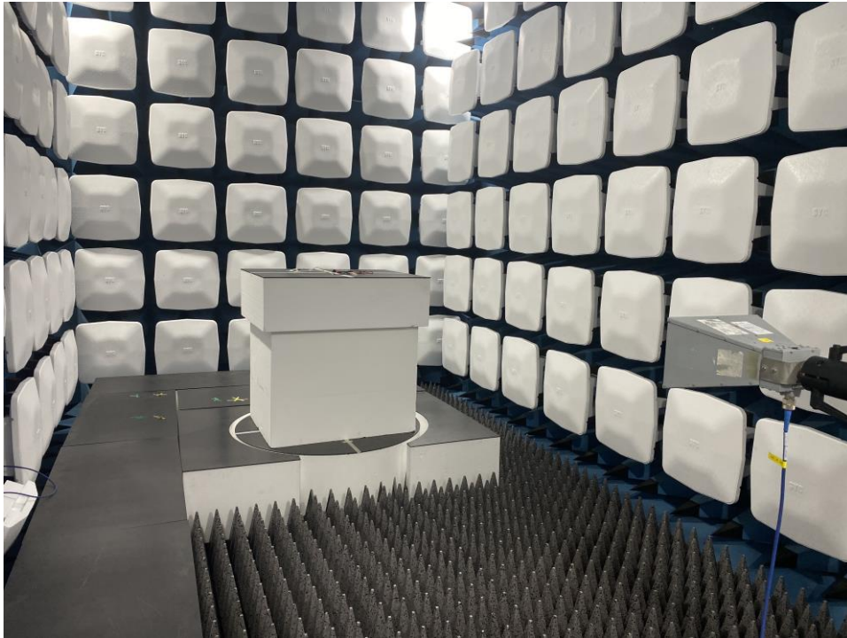
Left, Radiated Test_Above 1GHz_Rear
