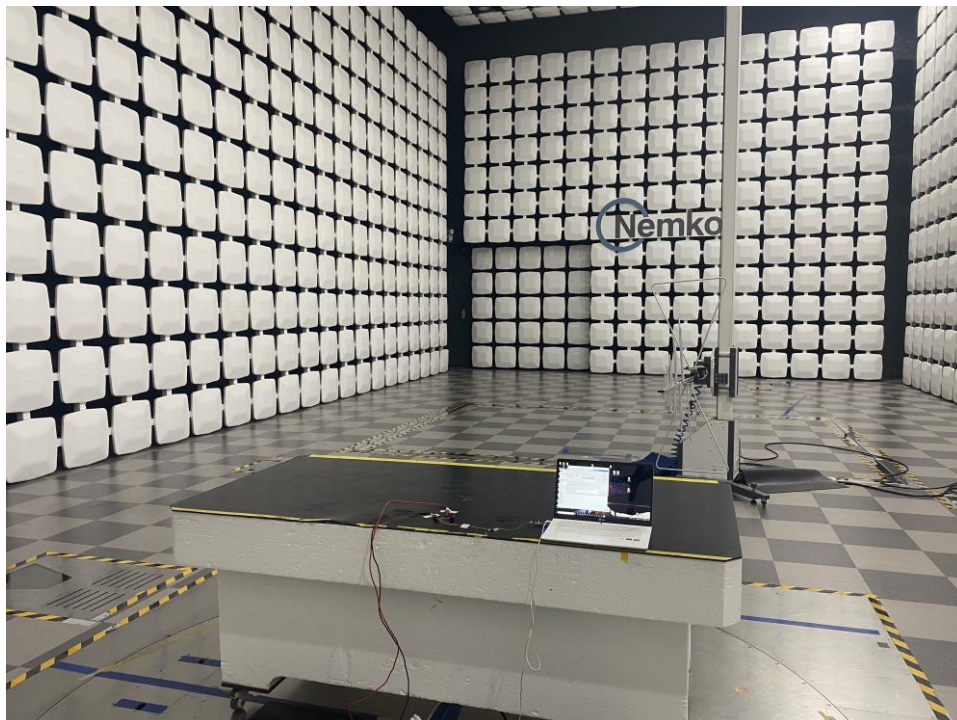
Right, Radiated Test_Below 1GHz_Rear
