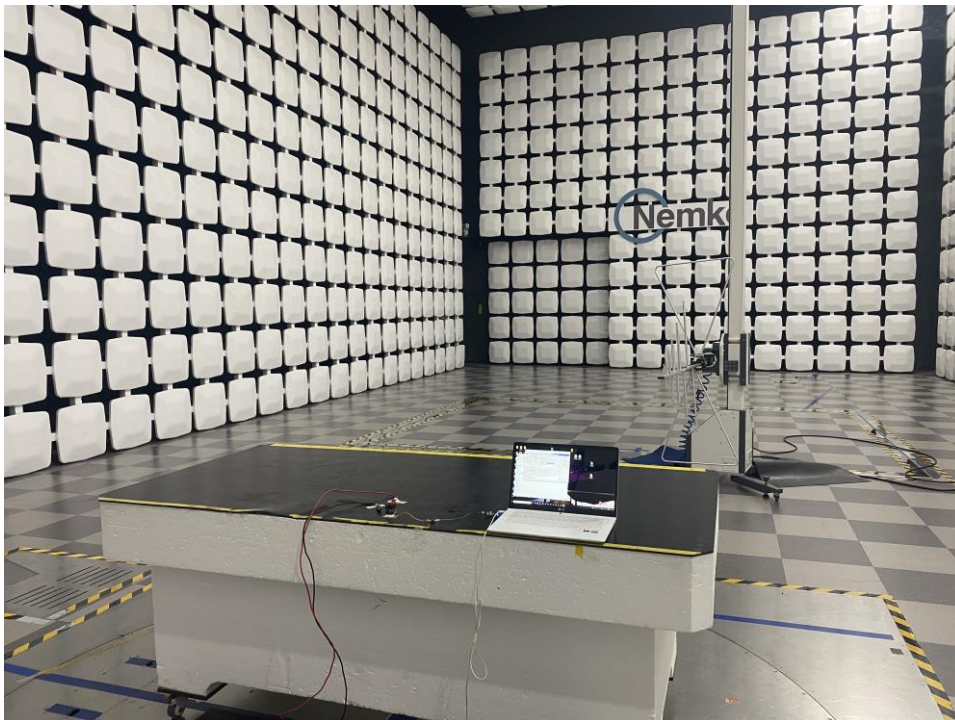
Left, Radiated Test_Below 1GHz_Rear
