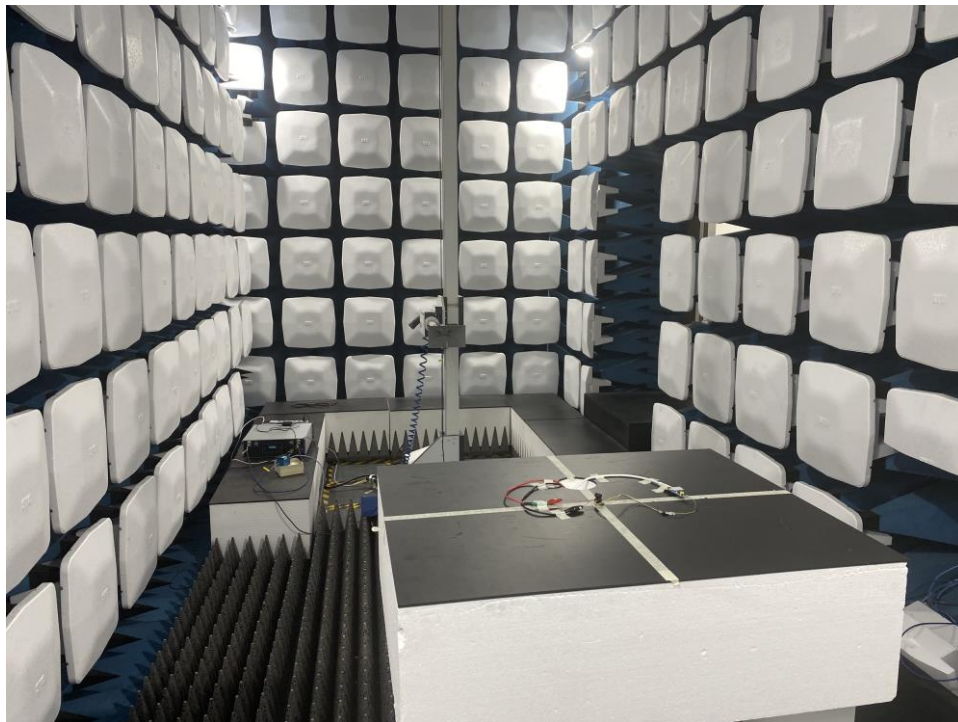
Right, Radiated Test_Above 1GHz_Rear
