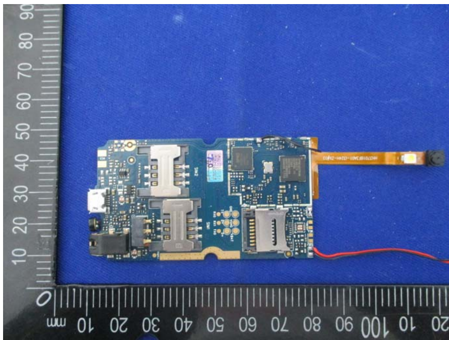
EUT –Main Board Top Unshiled View
