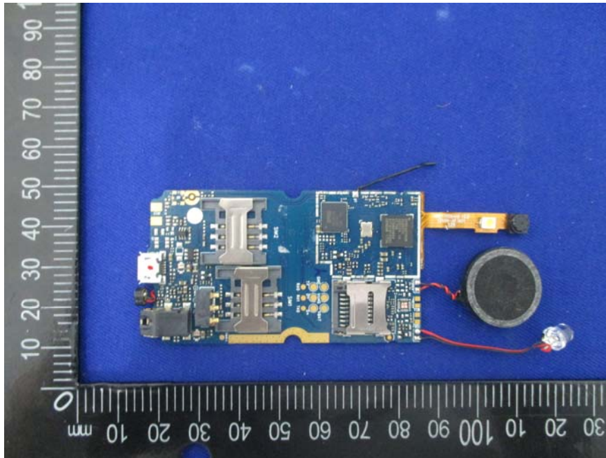
EUT –Mainboard Unshiled Top View
