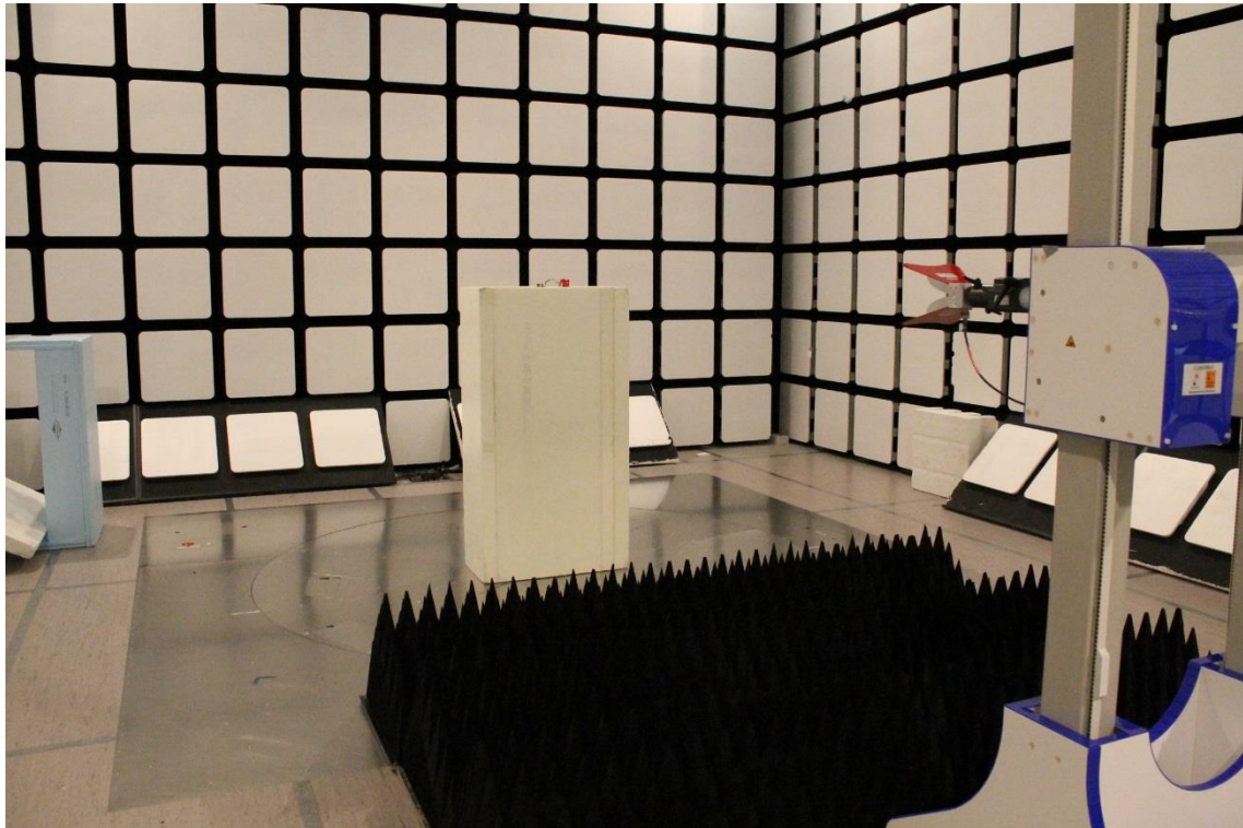
Photograph 5. Radiated Spurious Emissions 1 – 2 GHz
