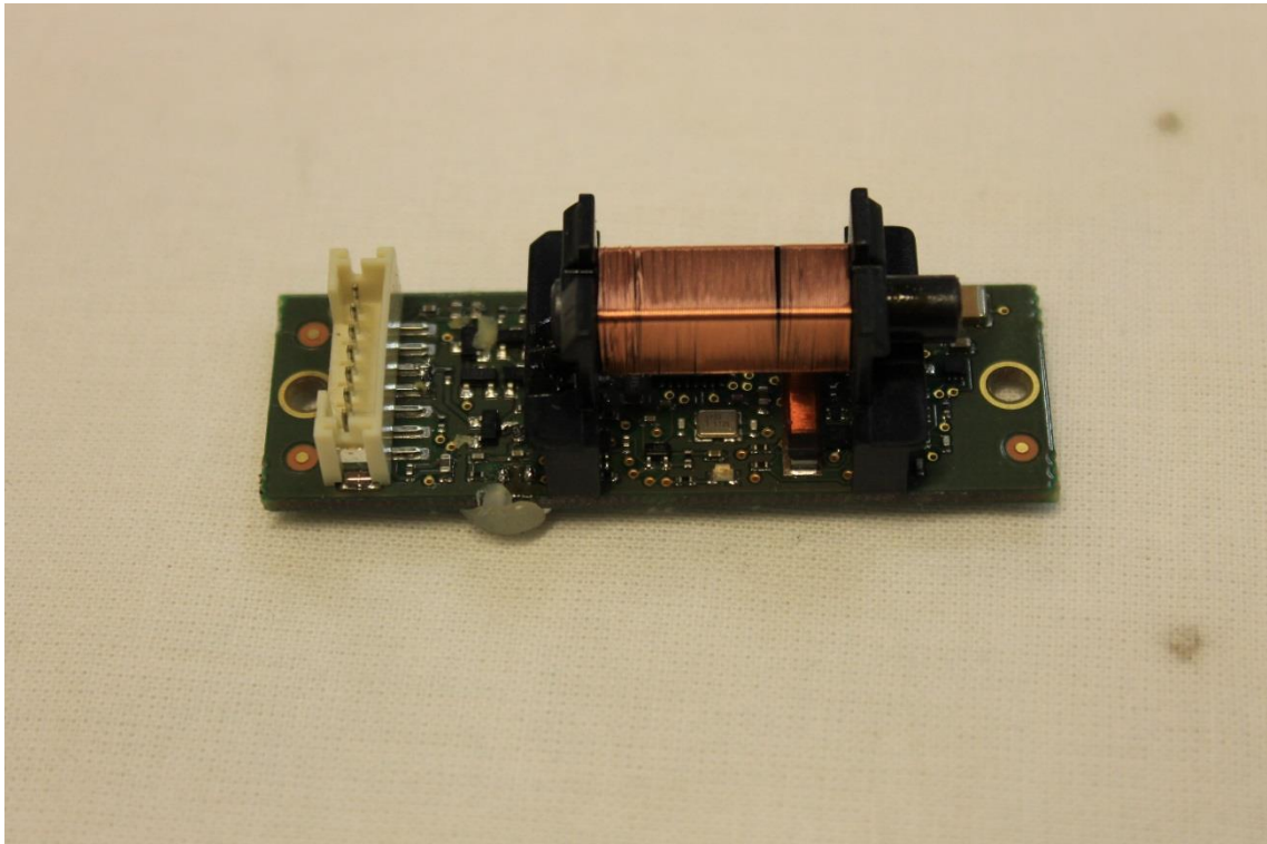
Photograph 1. DUT 1
