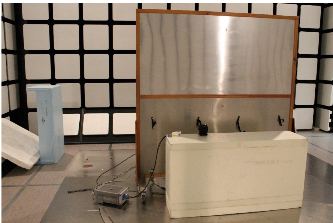
Photograph 8. Conducted spurious emissions test set-up
