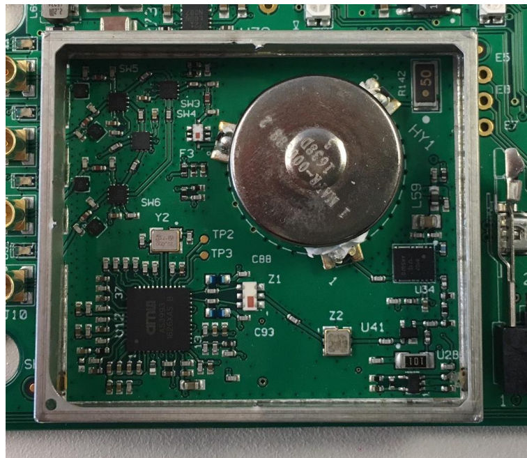
RF Section of EUT
