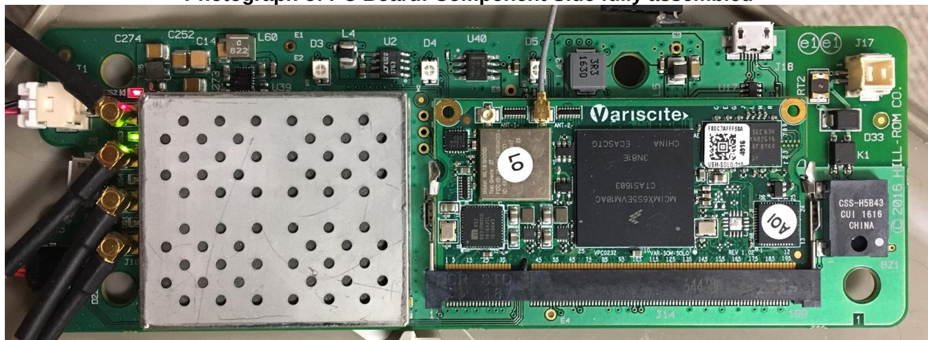
Photograph of PC Board: Component Side fully assembled
