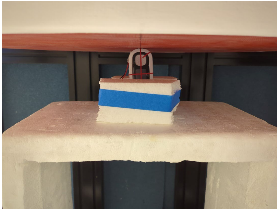
Photograph 7: Body-worn/Extremity, Edge Top, 0 mm
