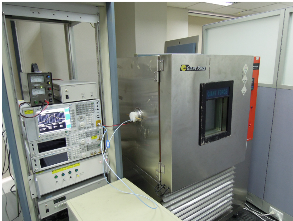
Photograph 9: Set-up for Conducted testing
