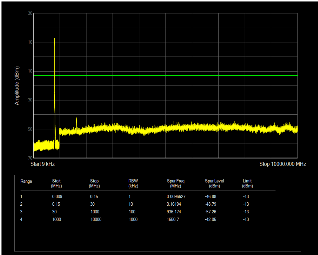
Band18 QPSK BW=10MHz Channel=23950 RB Size=50 Position=#0
