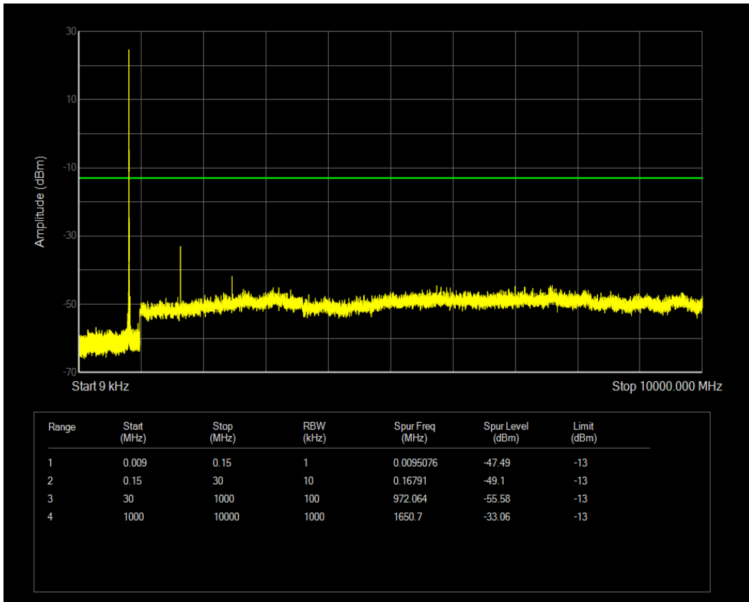
Band18 QAM16 BW=5MHz Channel=23975 RB Size=25 Position=#0
