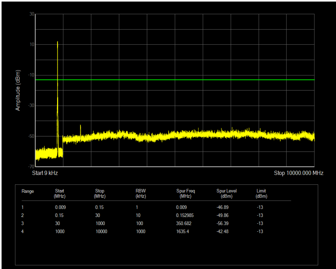
Band18 QPSK BW=10MHz Channel=23900 RB Size=50 Position=#0
