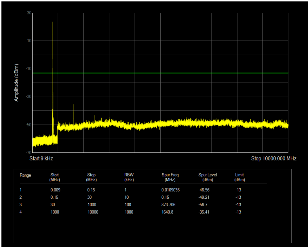
Band18 QPSK BW=10MHz Channel=23950 RB Size=50 Position=#0
