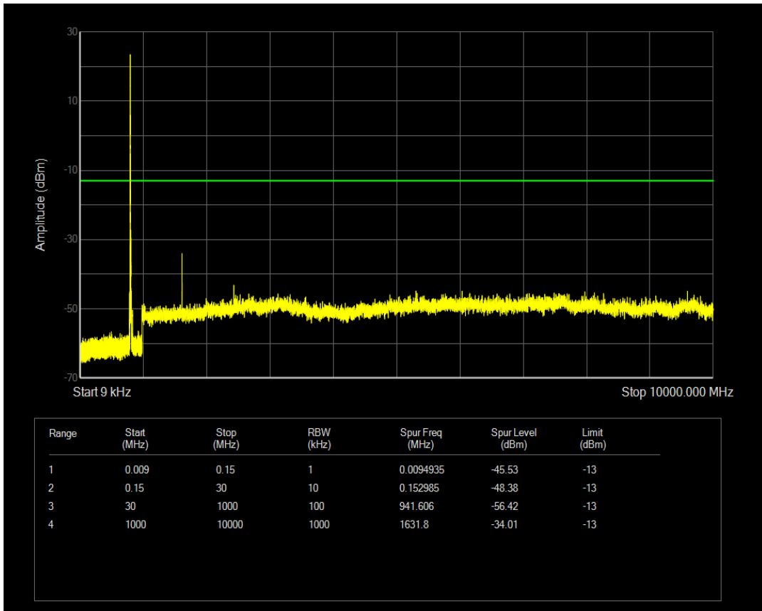
Band18 QPSK BW=10MHz Channel=23900 RB Size=50 Position=#0
