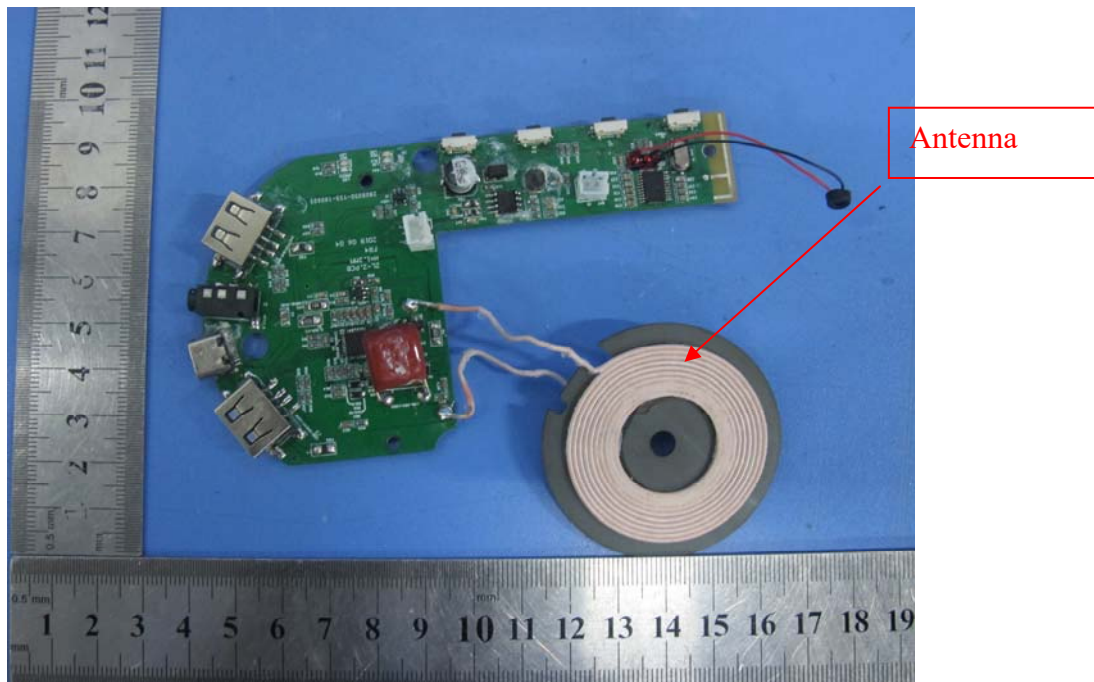
Photo 8 Appearance of PCB
