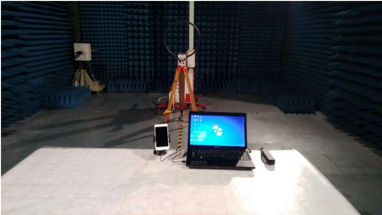
Photos of Radiated Emission Test
