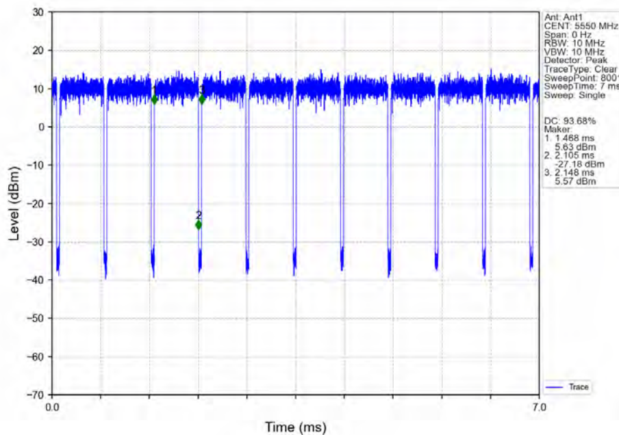
802.11n(HT40)_MCH_5550MHz_Ant1_NTNV
