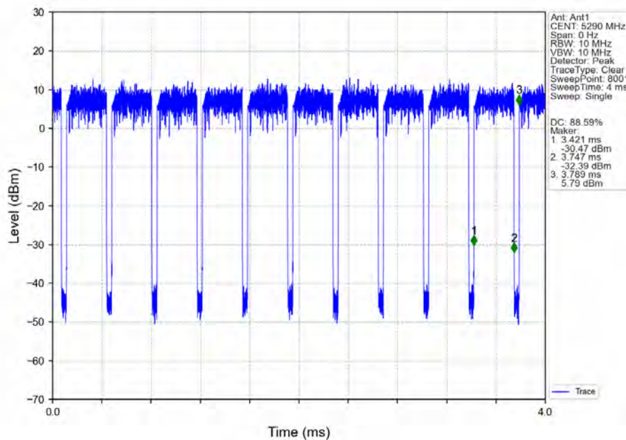
802.11ac(VHT80)_MCH_5290MHz_Ant1_NTNV
