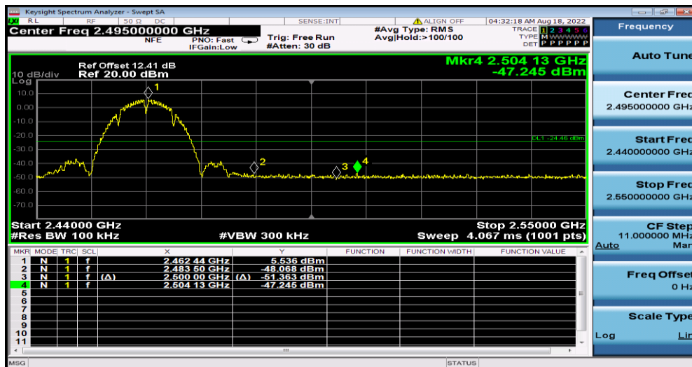
11B_Ant2_High_2462
