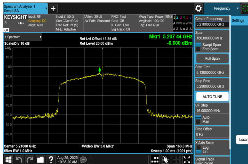
11AC80MIMO-Ant2-5210-PASS
