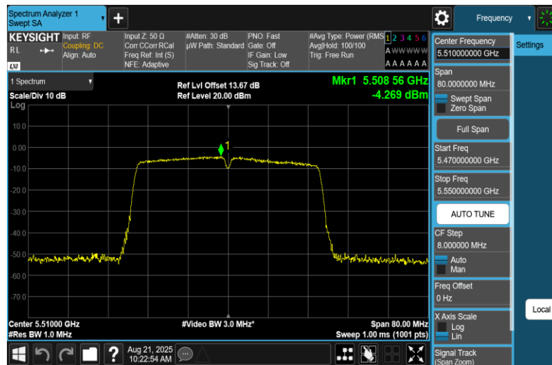
11AC40MIMO-Ant2-5510-PASS
