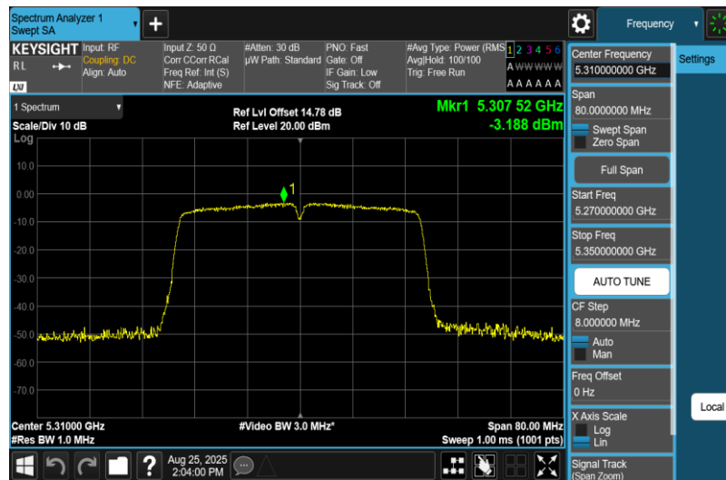
11AC40MIMO-Ant1-5310-PASS
