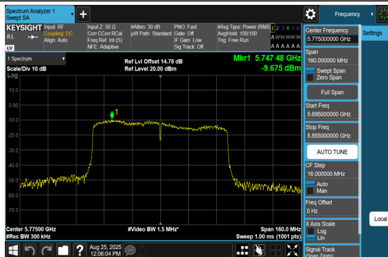
11AC80MIMO-Ant1-5775-PASS
