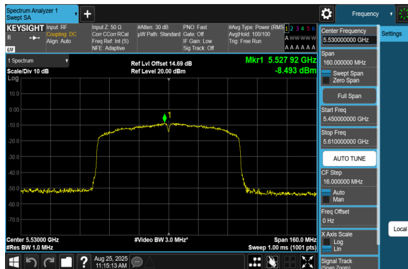
11AC80MIMO-Ant1-5530-PASS
