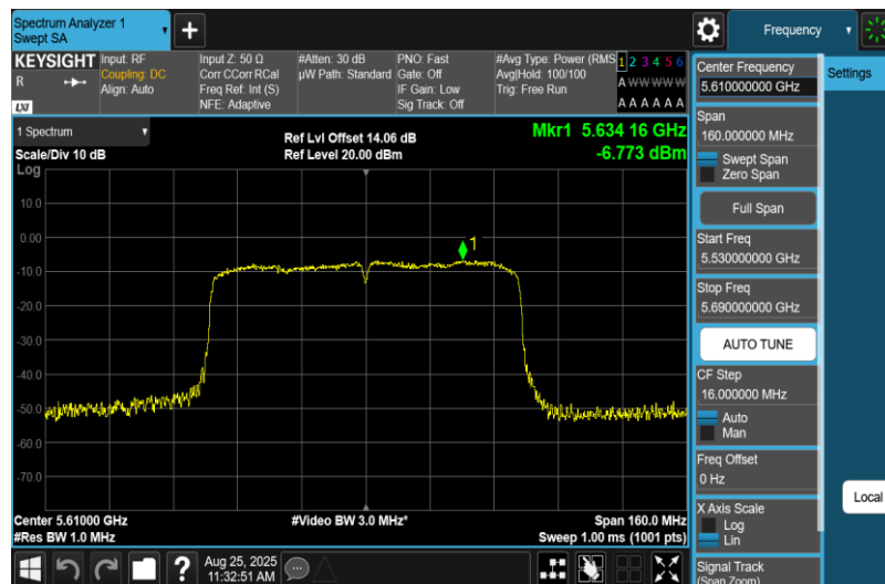
11AC80MIMO-Ant2-5610-PASS
