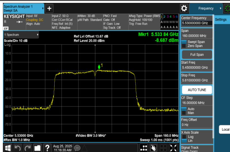
11AC80MIMO-Ant2-5530-PASS
