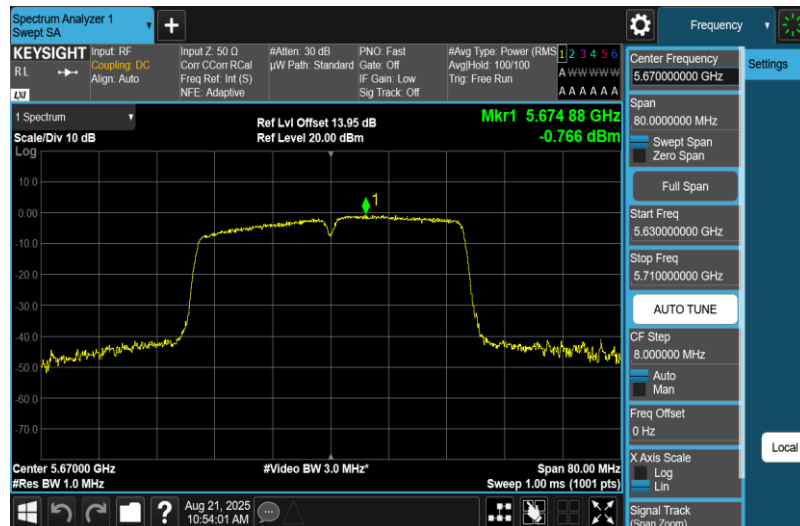
11AC40MIMO-Ant2-5670-PASS
