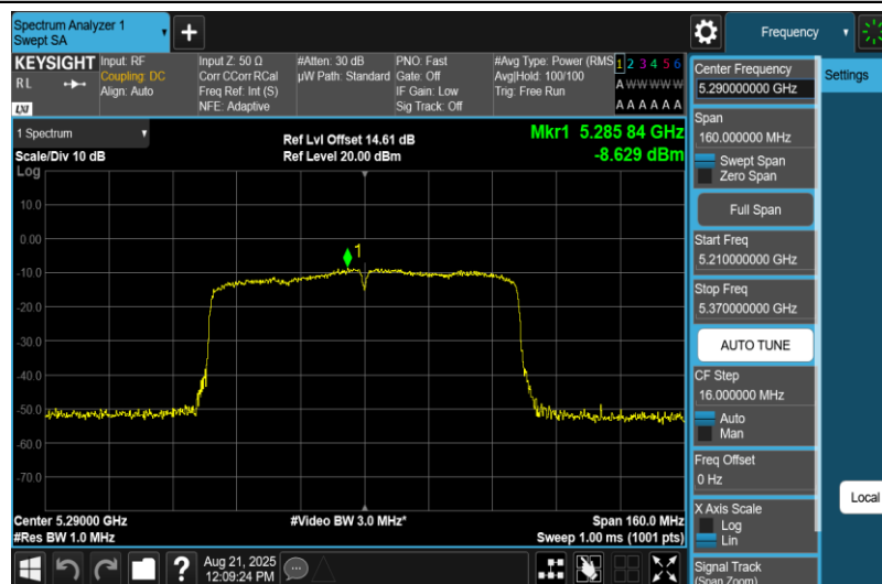
11AC80MIMO-Ant1-5290-PASS
