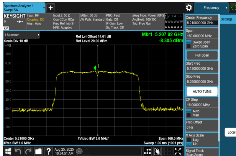
11AC80MIMO-Ant1-5210-PASS
