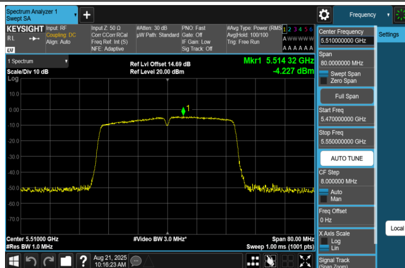
11AC40MIMO-Ant1-5510-PASS
