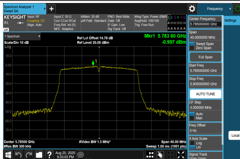
11AC20MIMO-Ant1-5785-PASS
