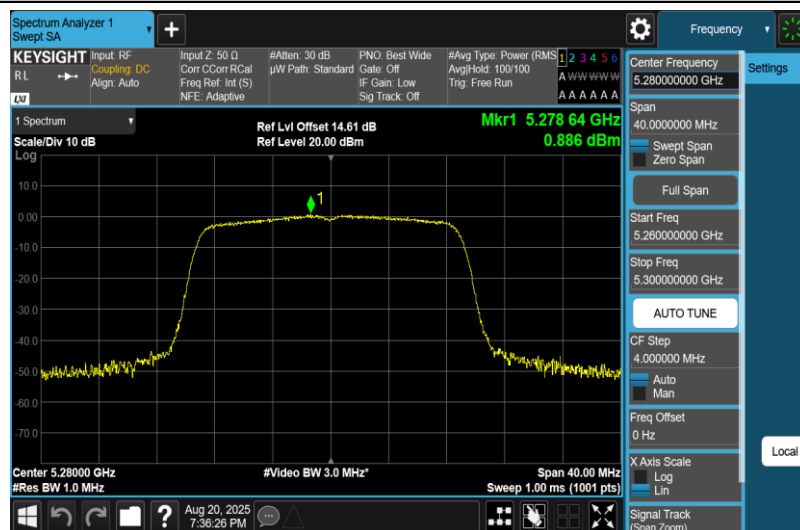
11AC20MIMO-Ant1-5280-PASS
