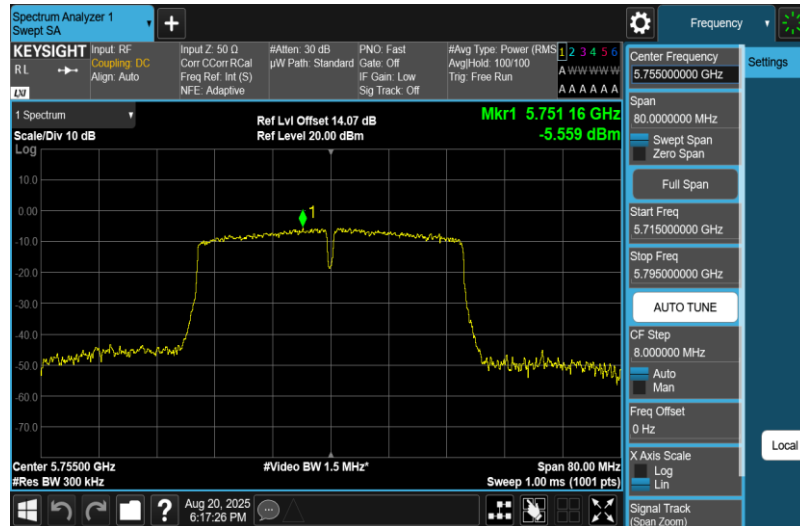
11N40MIMO-Ant2-5755-PASS
