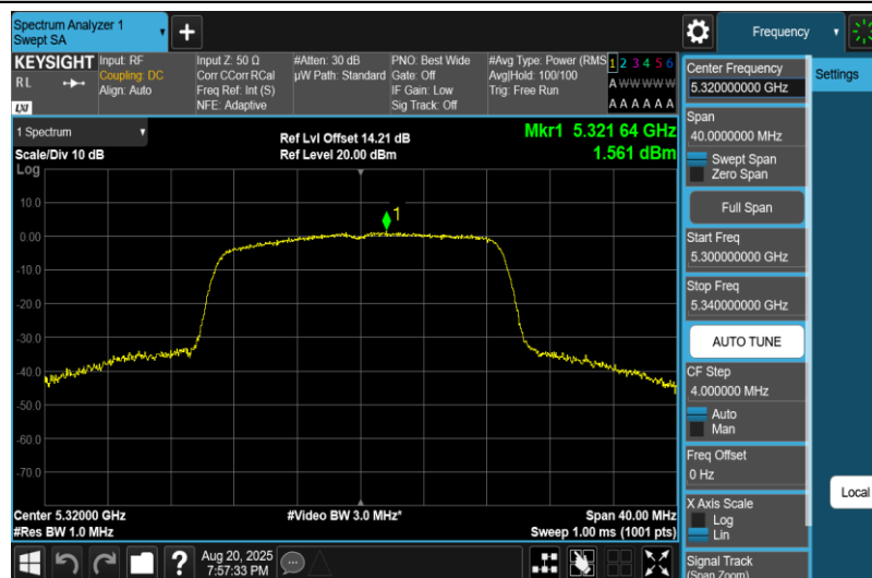
11AC20MIMO-Ant2-5320-PASS
