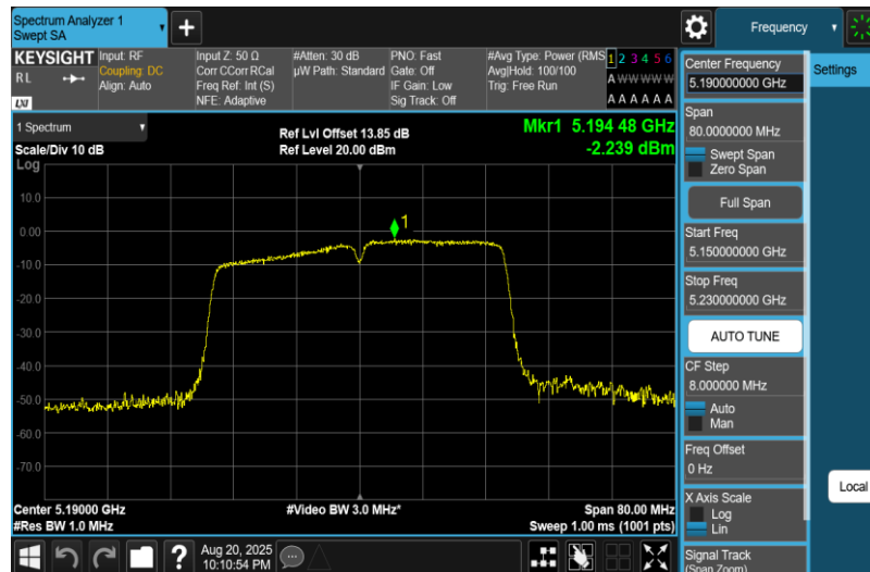
11AC40MIMO-Ant2-5190-PASS
