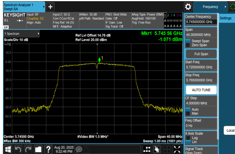
11AC20MIMO-Ant1-5745-PASS
