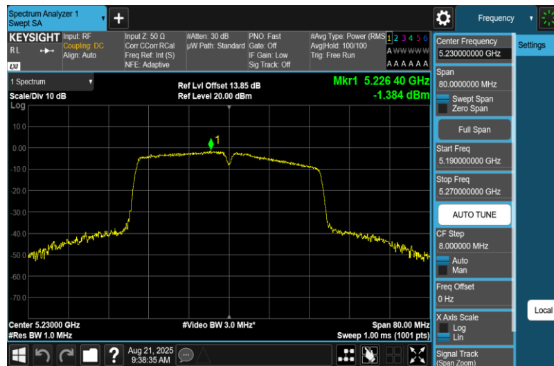
11AC40MIMO-Ant2-5230-PASS
