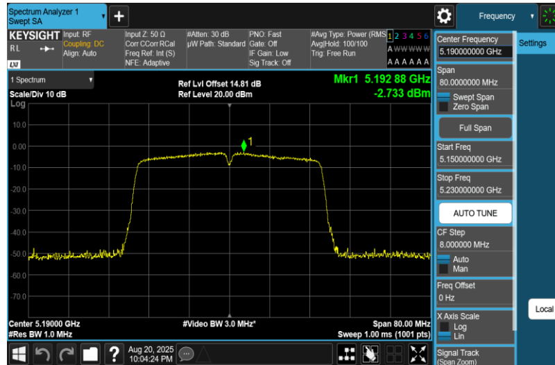
11AC40MIMO-Ant1-5190-PASS
