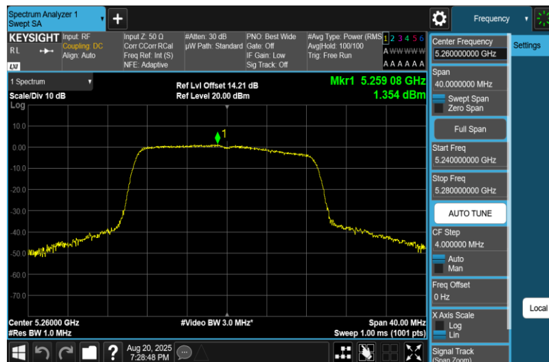
11AC20MIMO-Ant2-5260-PASS
