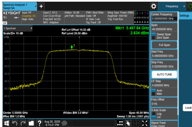
11AC20MIMO-Ant1-5500-PASS
