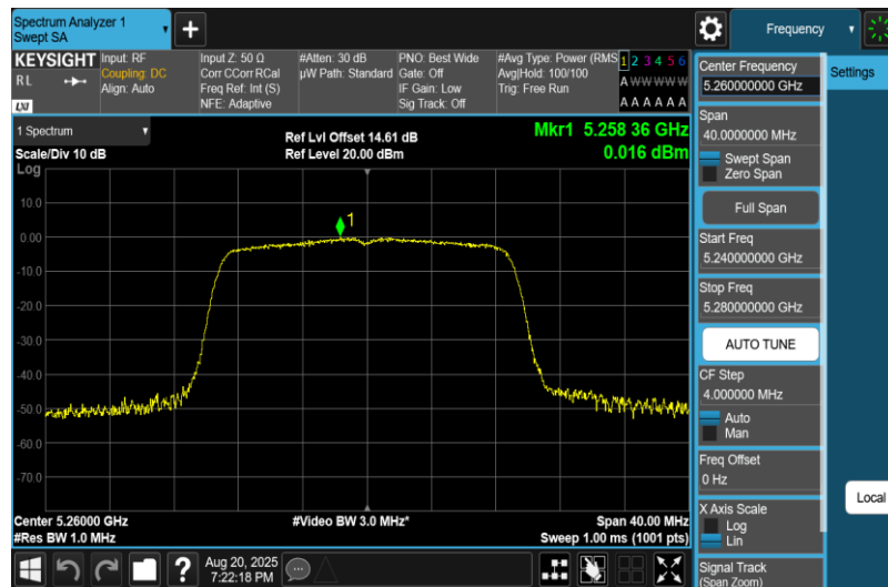
11AC20MIMO-Ant1-5260-PASS
