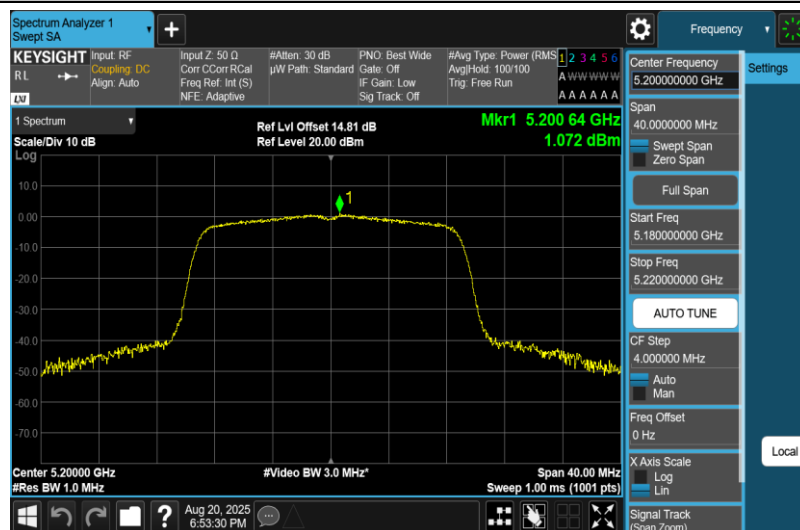
11AC20MIMO-Ant1-5200-PASS
