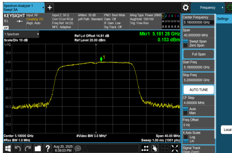
11AC20MIMO-Ant1-5180-PASS
