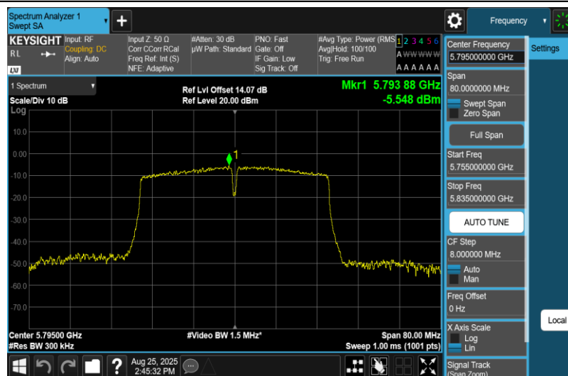
11N40MIMO-Ant2-5795-PASS
