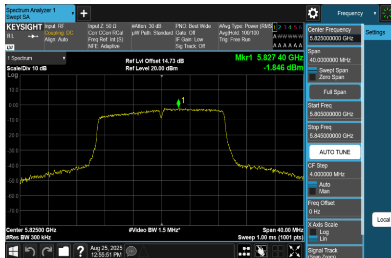
11AC20MIMO-Ant1-5825-PASS
