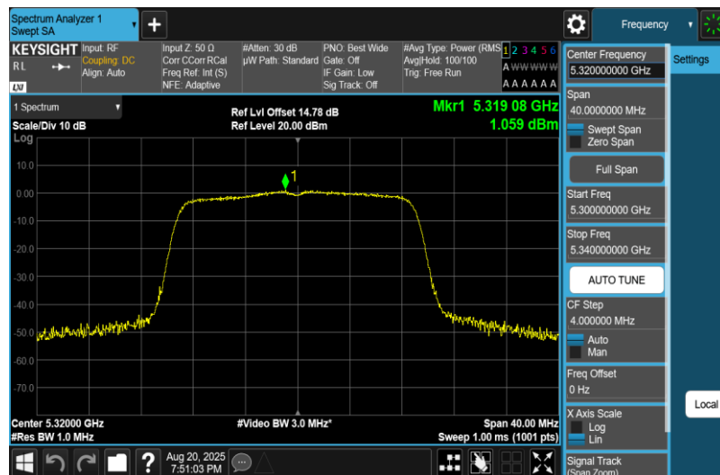
11AC20MIMO-Ant1-5320-PASS
