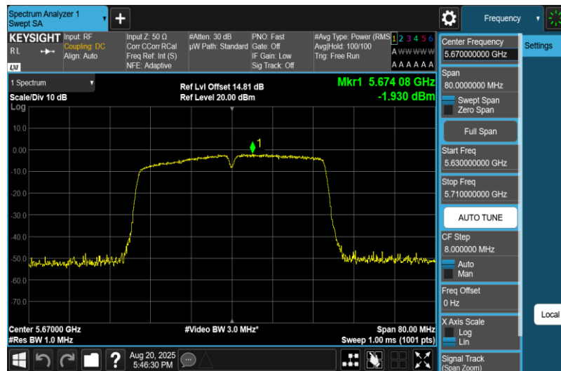
11N40MIMO-Ant1-5670-PASS
