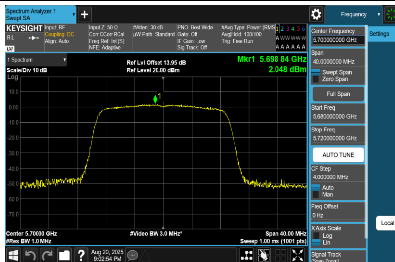
11AC20MIMO-Ant2-5700-PASS
