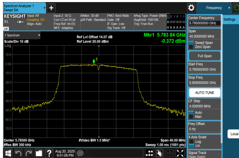
11AC20MIMO-Ant2-5785-PASS
