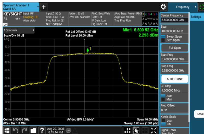
11AC20MIMO-Ant2-5500-PASS
