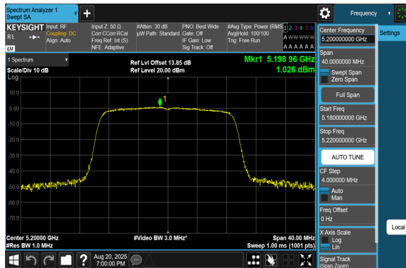
11AC20MIMO-Ant2-5200-PASS
