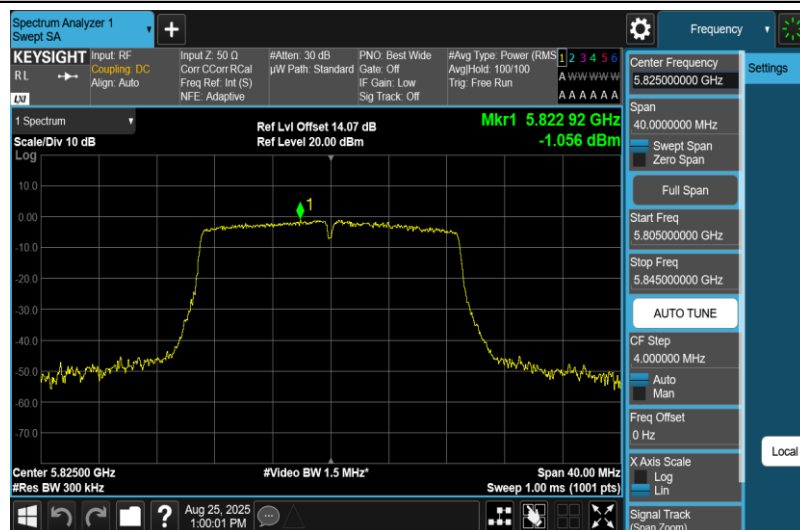
11AC20MIMO-Ant2-5825-PASS
