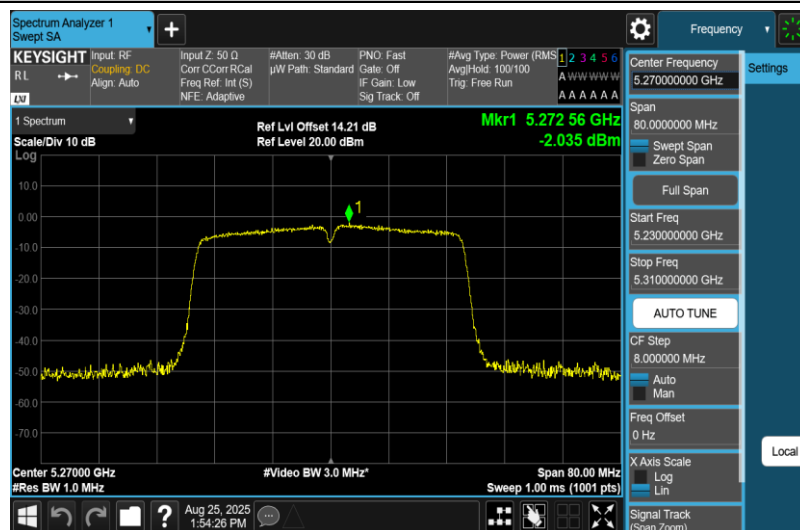
11AC40MIMO-Ant2-5270-PASS
