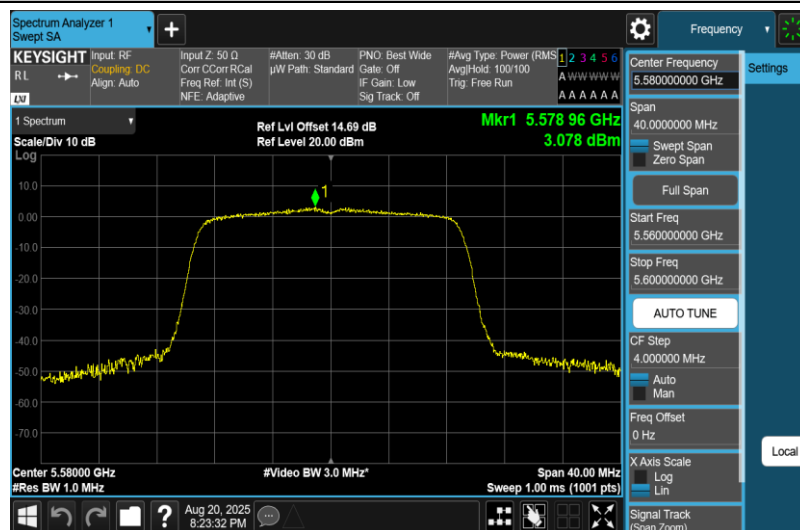
11AC20MIMO-Ant1-5580-PASS
