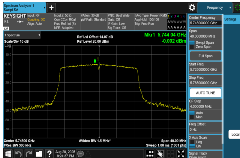
11AC20MIMO-Ant2-5745-PASS
