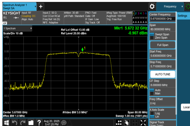
11N40MIMO-Ant2-5670-PASS
