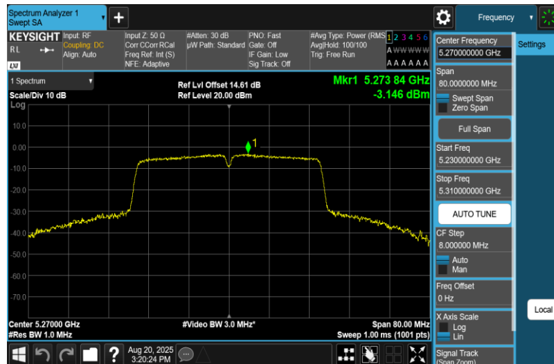
11N40MIMO-Ant1-5270-PASS
