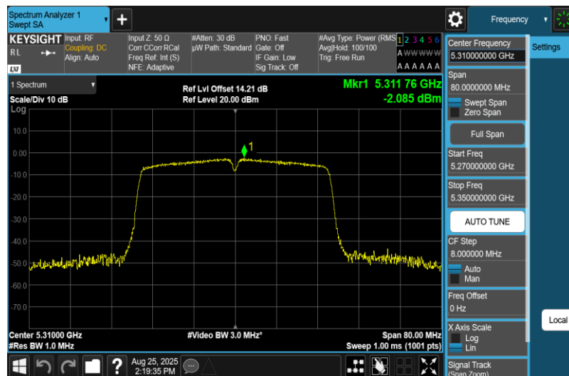
11N40MIMO-Ant2-5310-PASS
