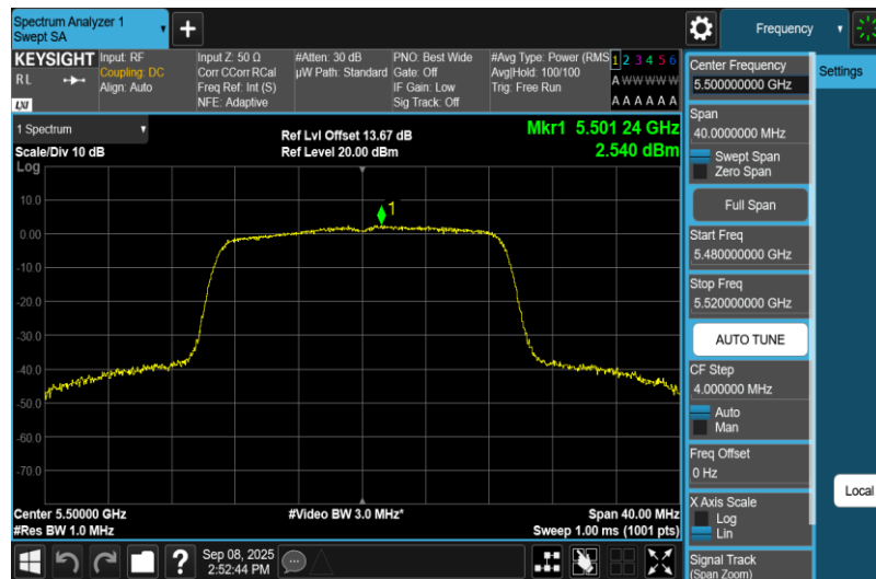
11N20MIMO-Ant2-5500-PASS
