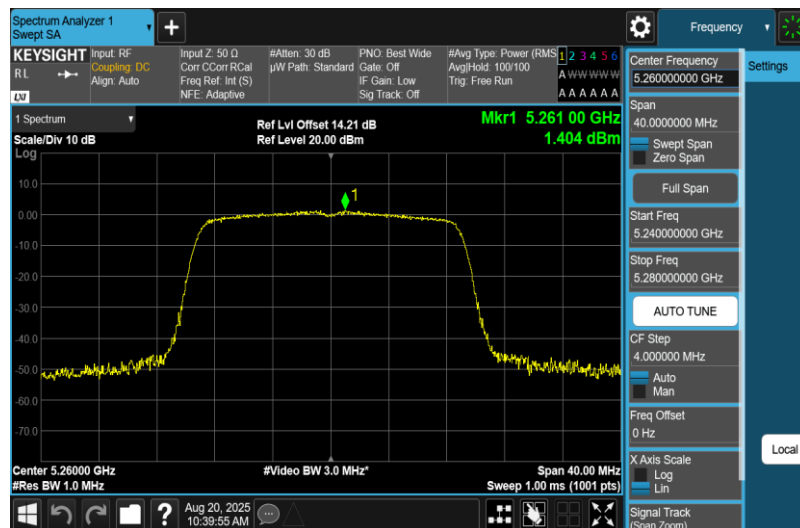
11N20MIMO-Ant2-5260-PASS
