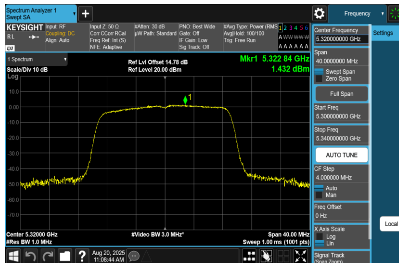
11N20MIMO-Ant1-5320-PASS
