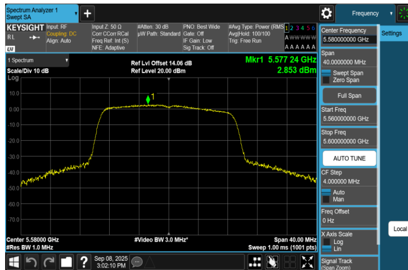
11N20MIMO-Ant2-5580-PASS
