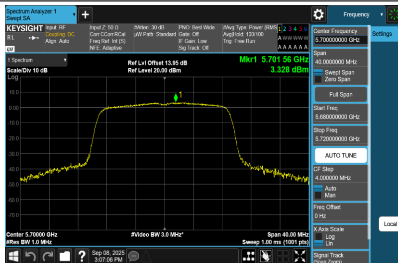
11N20MIMO-Ant2-5700-PASS
