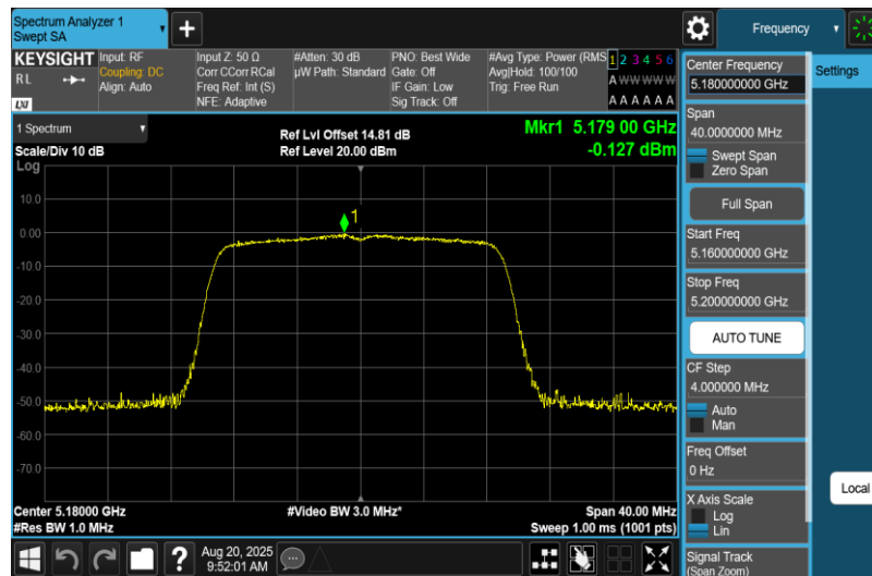
11N20MIMO-Ant1-5180-PASS
