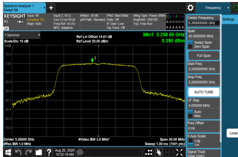
11N20MIMO-Ant1-5260-PASS
