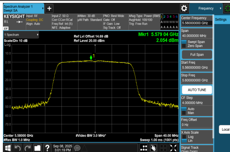
11N20MIMO-Ant1-5580-PASS
