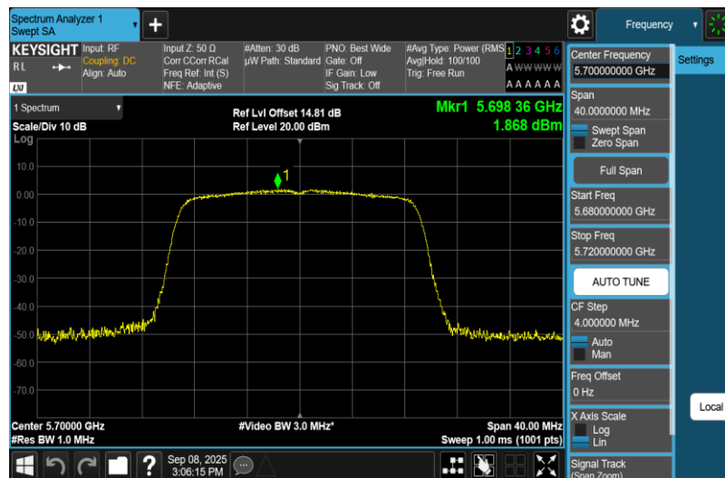
11N20MIMO-Ant1-5700-PASS
