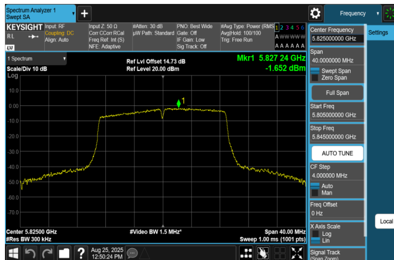
11N20MIMO-Ant1-5825-PASS
