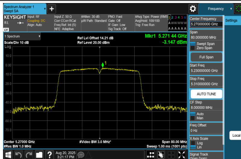
11N40MIMO-Ant2-5270-PASS
