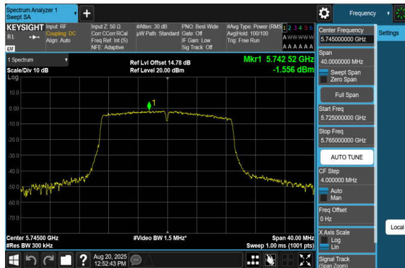
11N20MIMO-Ant1-5745-PASS
