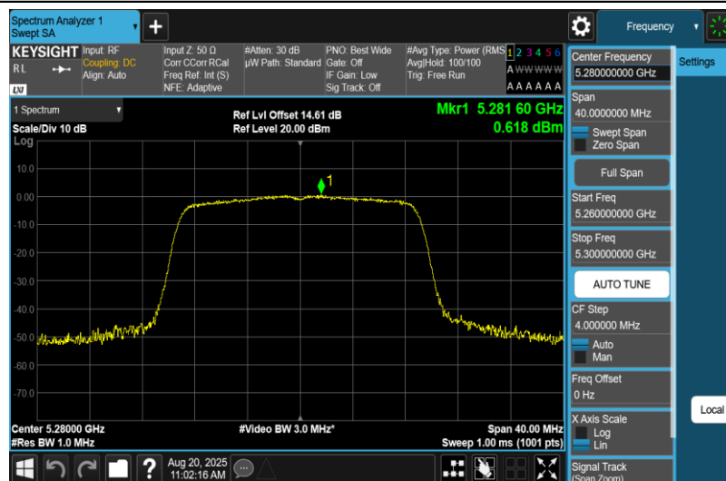
11N20MIMO-Ant1-5280-PASS
