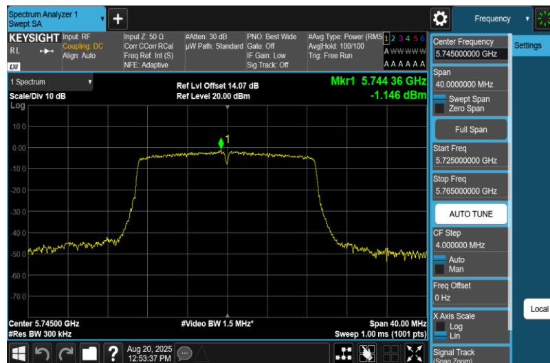
11N20MIMO-Ant2-5745-PASS
