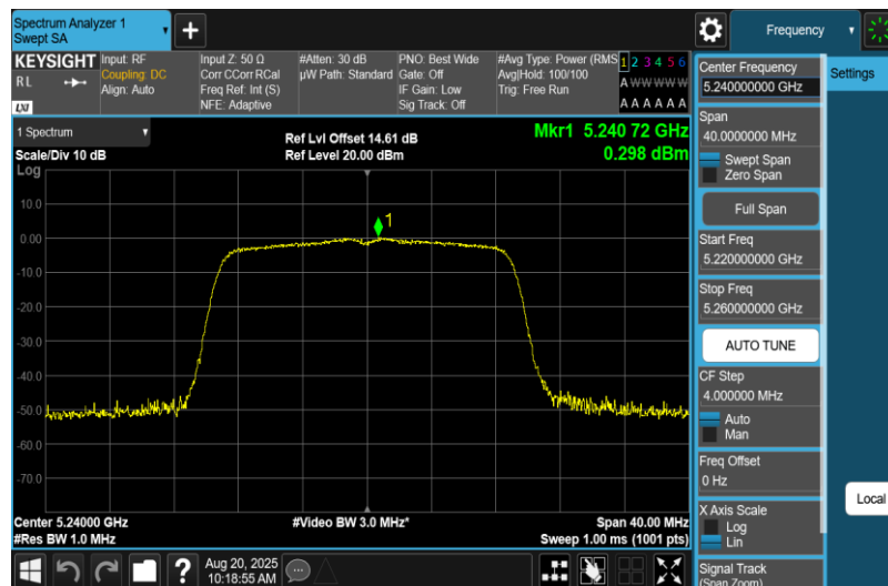
11N20MIMO-Ant1-5240-PASS
