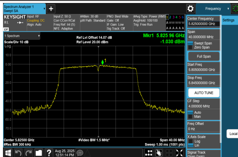
11N20MIMO-Ant2-5825-PASS
