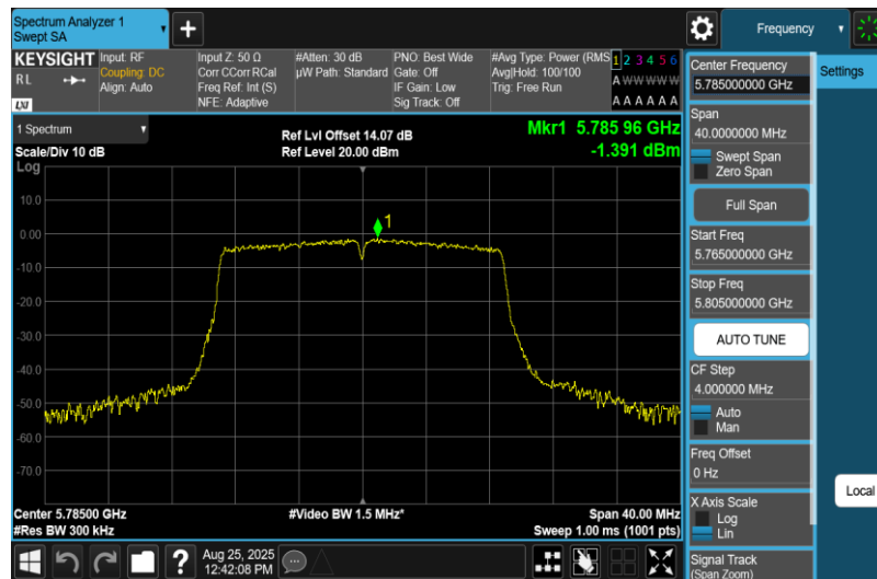
11N20MIMO-Ant2-5785-PASS
