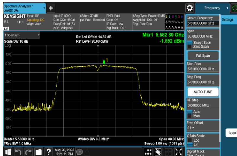
11N40MIMO-Ant1-5550-PASS
