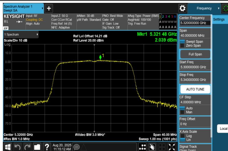
11N20MIMO-Ant2-5320-PASS
