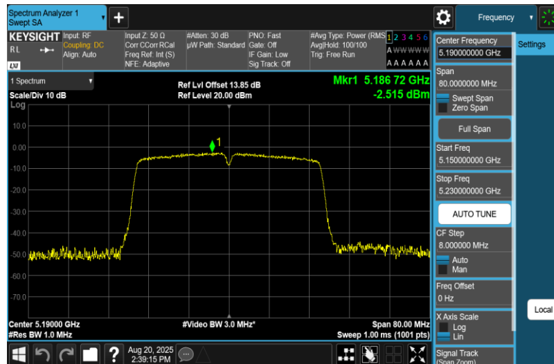
11N40MIMO-Ant2-5190-PASS
