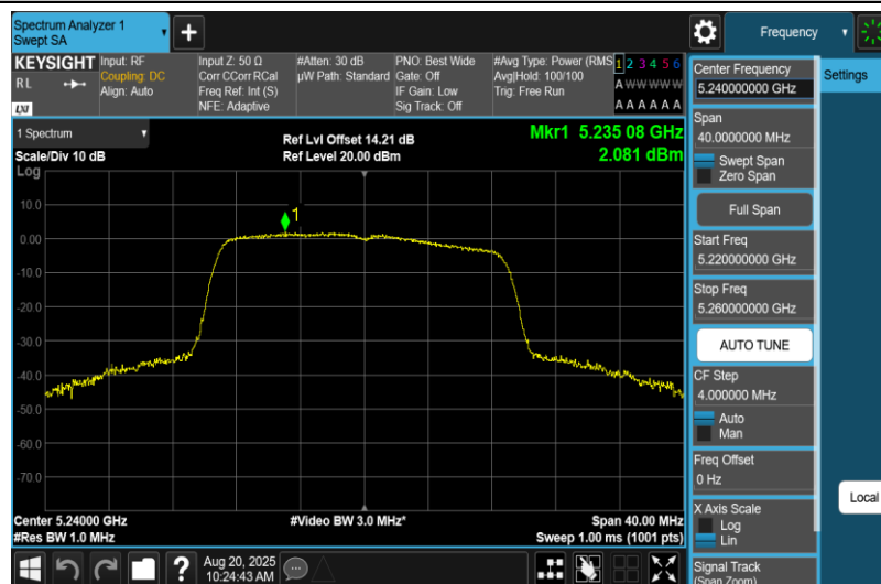
11N20MIMO-Ant2-5240-PASS
