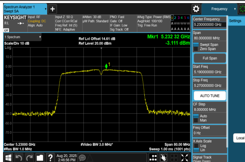
11N40MIMO-Ant1-5230-PASS
