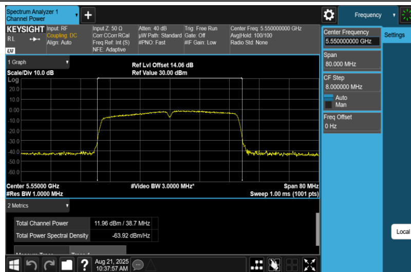
11AC40MIMO-Ant2-5550-PASS
