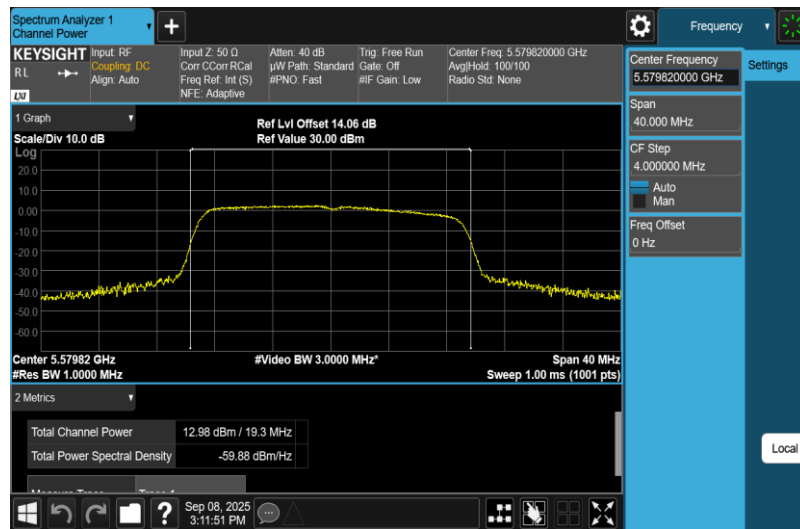
11AC20MIMO-Ant2-5580-PASS
