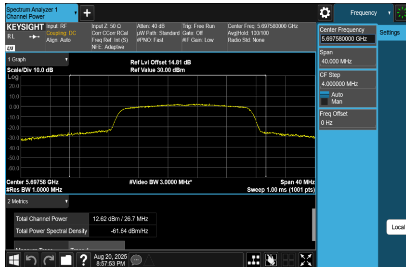
11AC20MIMO-Ant1-5700-PASS
