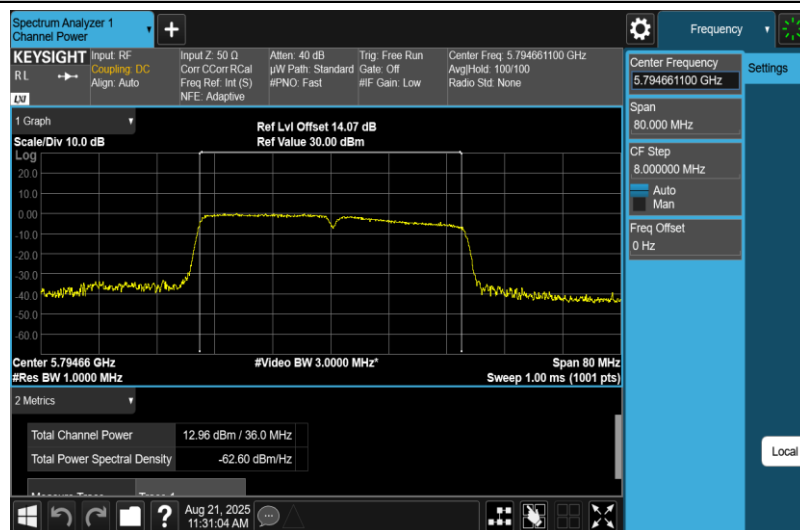
11AC40MIMO-Ant2-5795-PASS
