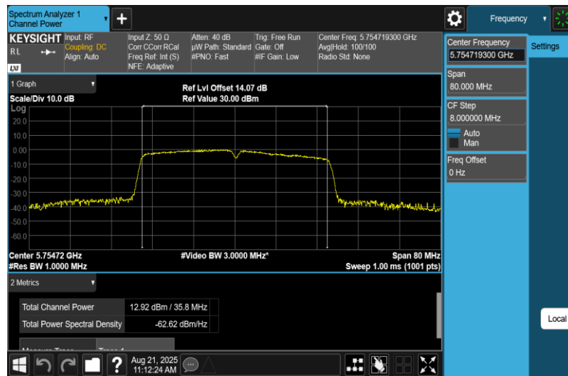
11AC40MIMO-Ant2-5755-PASS
