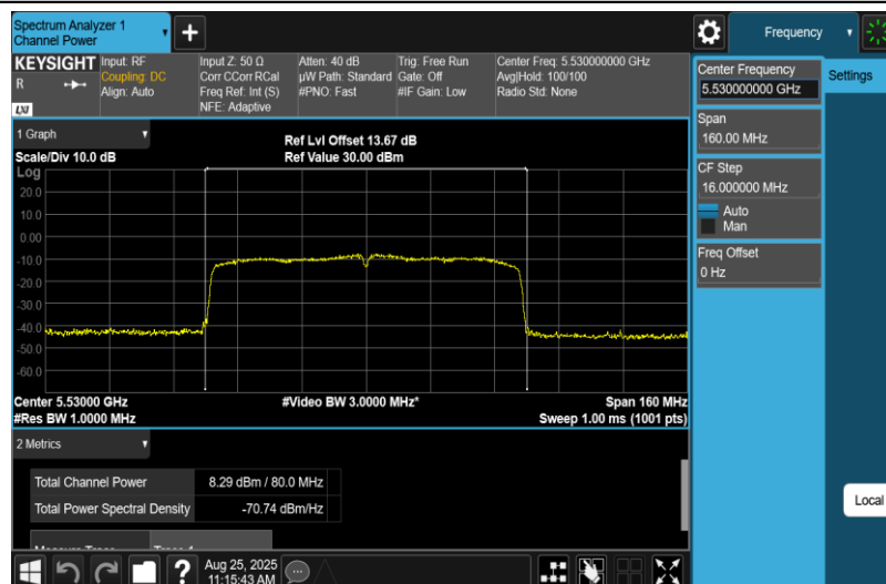
11AC80MIMO-Ant2-5530-PASS
