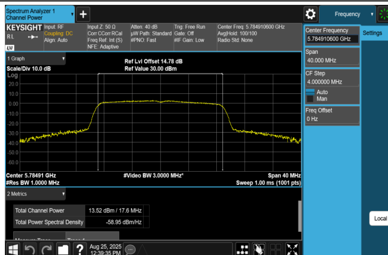
11N20MIMO-Ant1-5785-PASS
