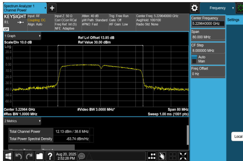
11N40MIMO-Ant2-5230-PASS
