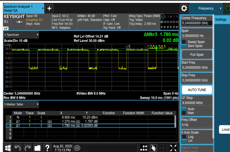
NTNV-11AC20MIMO-Ant2-5240
