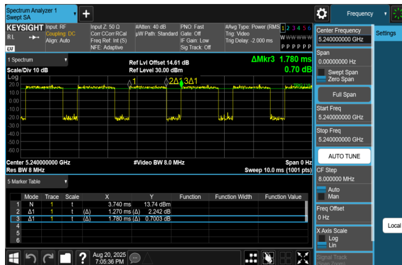
NTNV-11AC20MIMO-Ant1-5240
