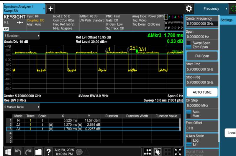
NTNV-11AC20MIMO-Ant2-5700
