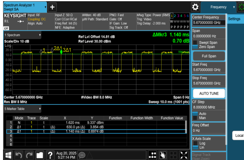
NTNV-11N40MIMO-Ant1-5670
