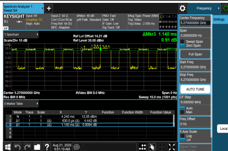
NTNV-11AC40MIMO-Ant2-5270
