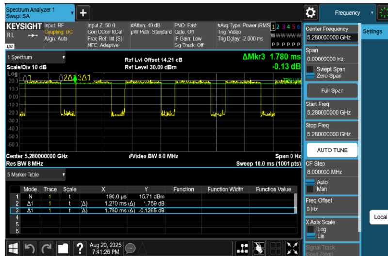
NTNV-11AC20MIMO-Ant2-5280
