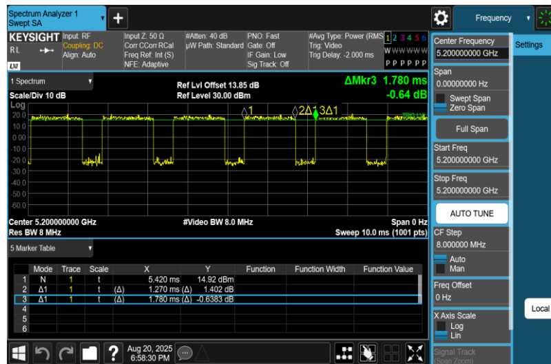
NTNV-11AC20MIMO-Ant2-5200
