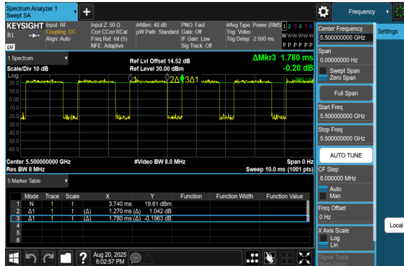
NTNV-11AC20MIMO-Ant1-5500
