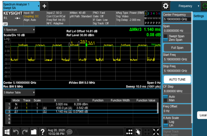
NTNV-11AC40MIMO-Ant1-5190
