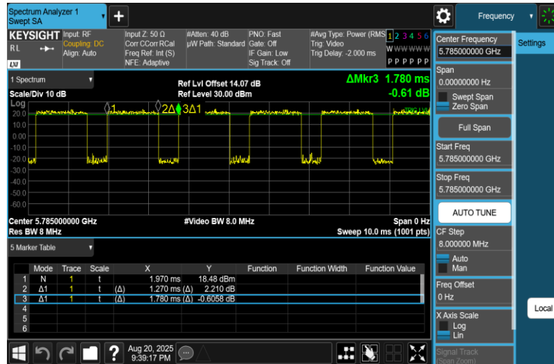
NTNV-11AC20MIMO-Ant2-5785
