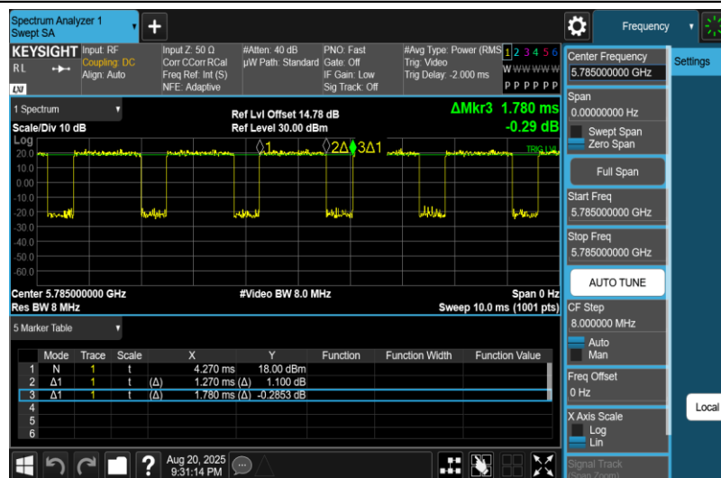
NTNV-11AC20MIMO-Ant1-5785
