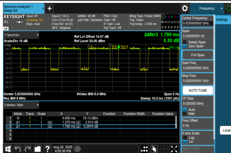
NTNV-11AC20MIMO-Ant2-5825
