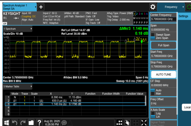
NTNV-11N40MIMO-Ant2-5795
