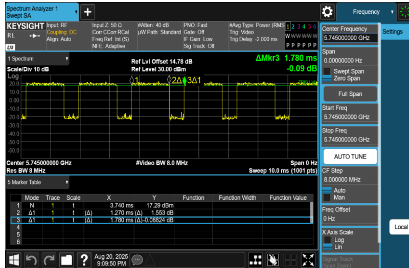
NTNV-11AC20MIMO-Ant1-5745
