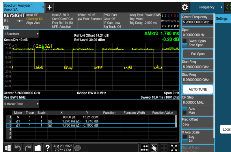
NTNV-11AC20MIMO-Ant2-5260
