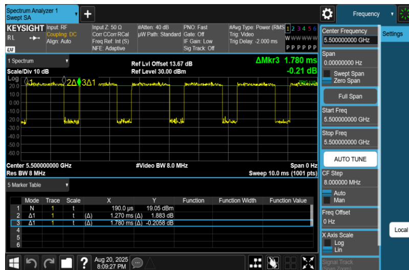
NTNV-11AC20MIMO-Ant2-5500
