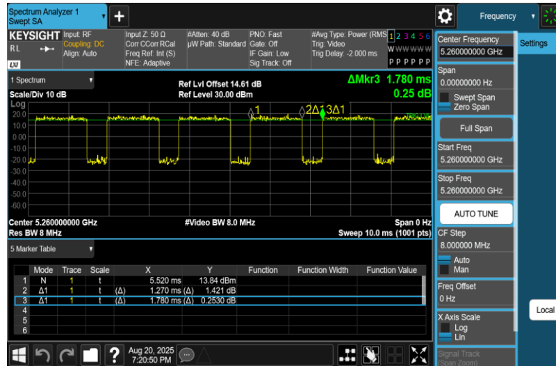
NTNV-11AC20MIMO-Ant1-5260
