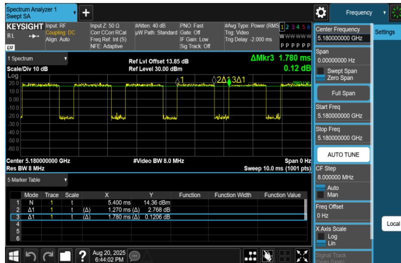
NTNV-11AC20MIMO-Ant2-5180
