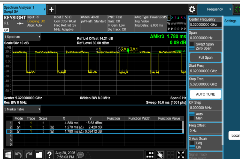
NTNV-11AC20MIMO-Ant2-5320
