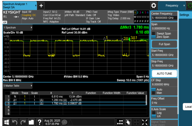
NTNV-11AC20MIMO-Ant1-5180
