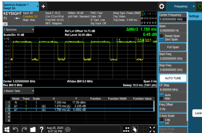
NTNV-11AC20MIMO-Ant1-5825
