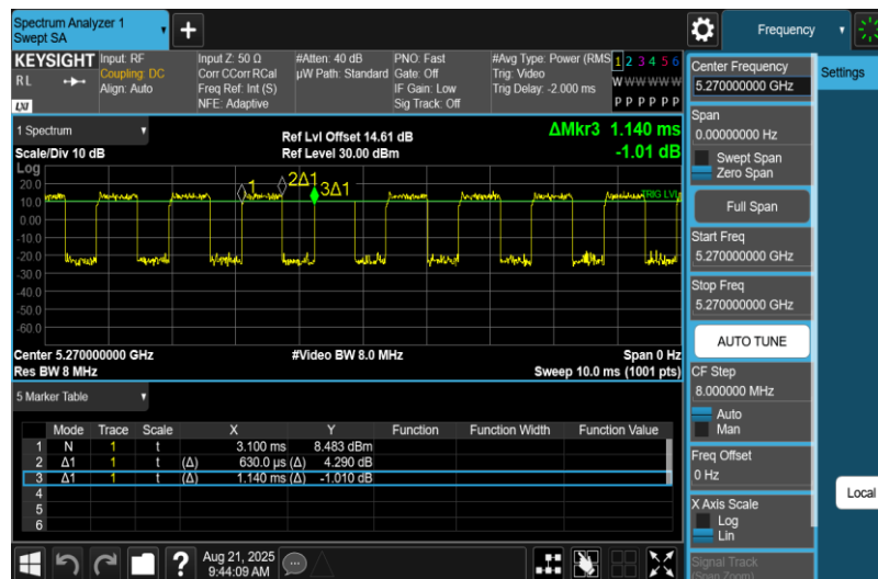
NTNV-11AC40MIMO-Ant1-5270
