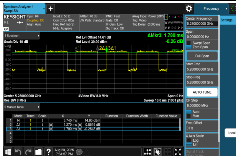
NTNV-11AC20MIMO-Ant1-5280
