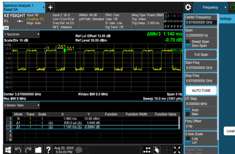
NTNV-11N40MIMO-Ant2-5670
