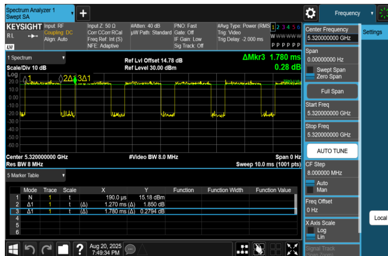
NTNV-11AC20MIMO-Ant1-5320
