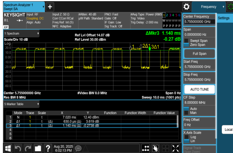
NTNV-11N40MIMO-Ant2-5755
