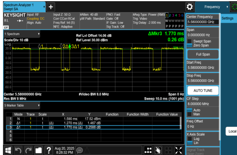
NTNV-11AC20MIMO-Ant2-5580
