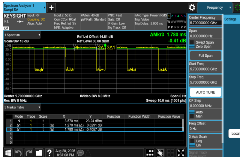
NTNV-11AC20MIMO-Ant1-5700
