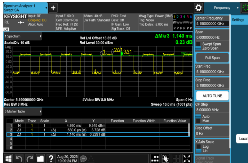
NTNV-11AC40MIMO-Ant2-5190
