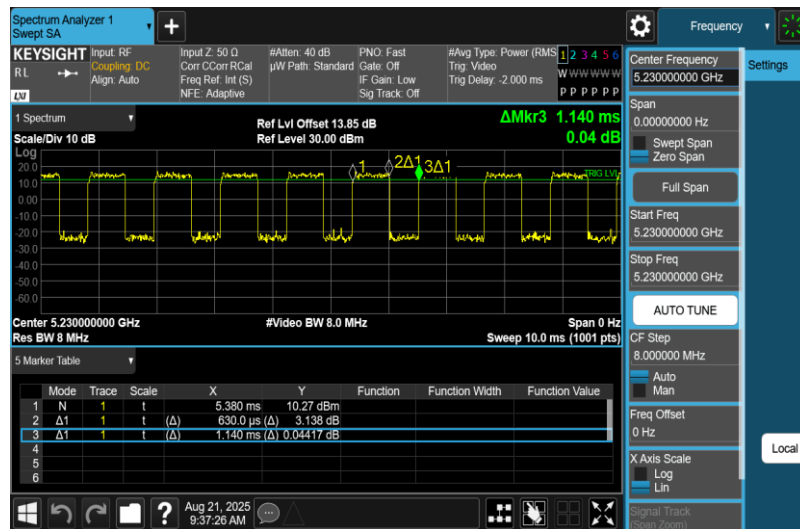
NTNV-11AC40MIMO-Ant2-5230
