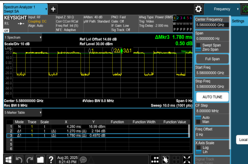
NTNV-11AC20MIMO-Ant1-5580
