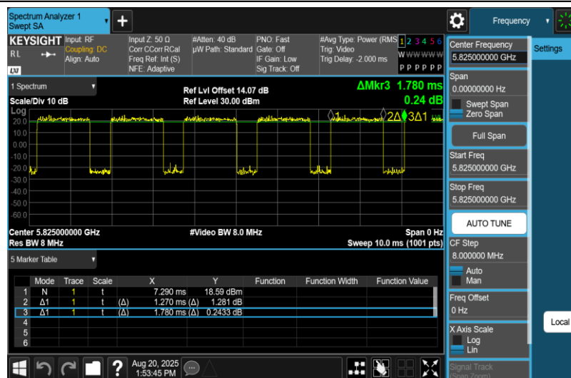
NTNV-11N20MIMO-Ant2-5825
