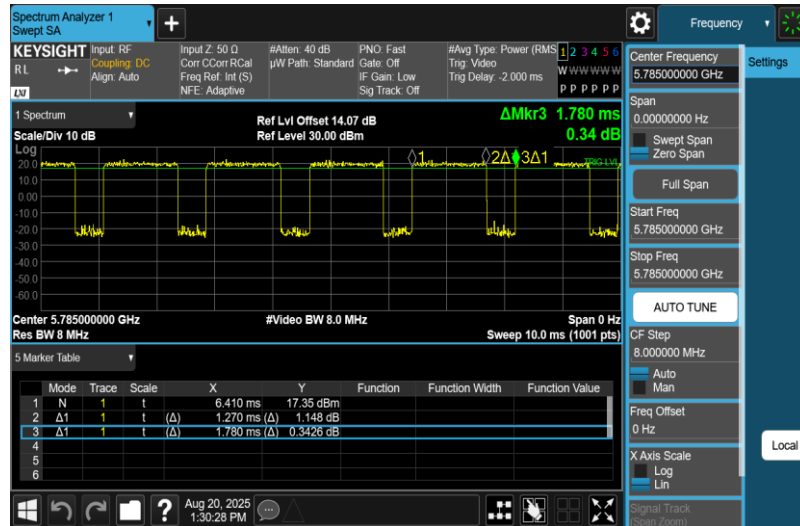
NTNV-11N20MIMO-Ant2-5785
