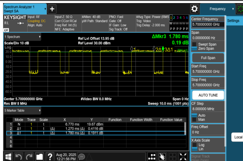
NTNV-11N20MIMO-Ant2-5700
