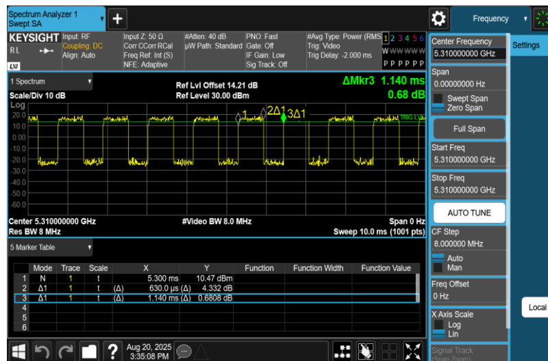
NTNV-11N40MIMO-Ant2-5310
