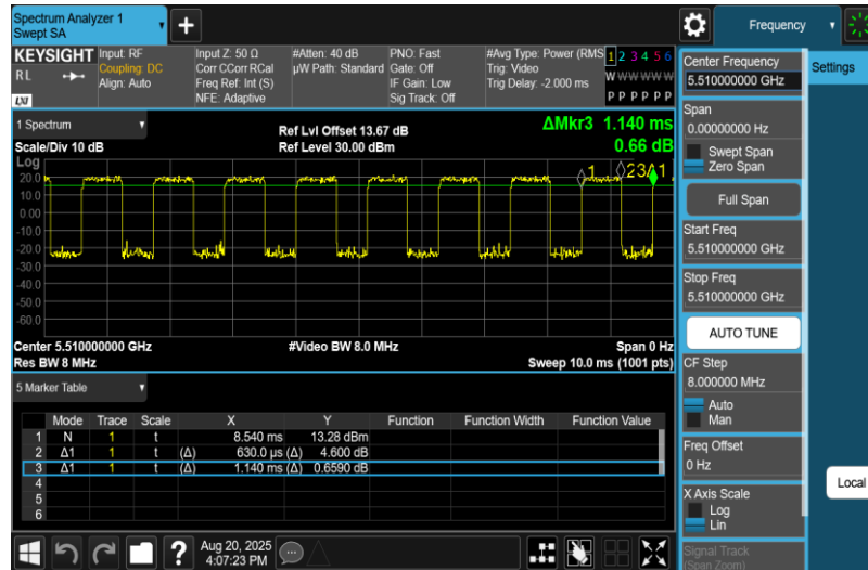
NTNV-11N40MIMO-Ant2-5510
