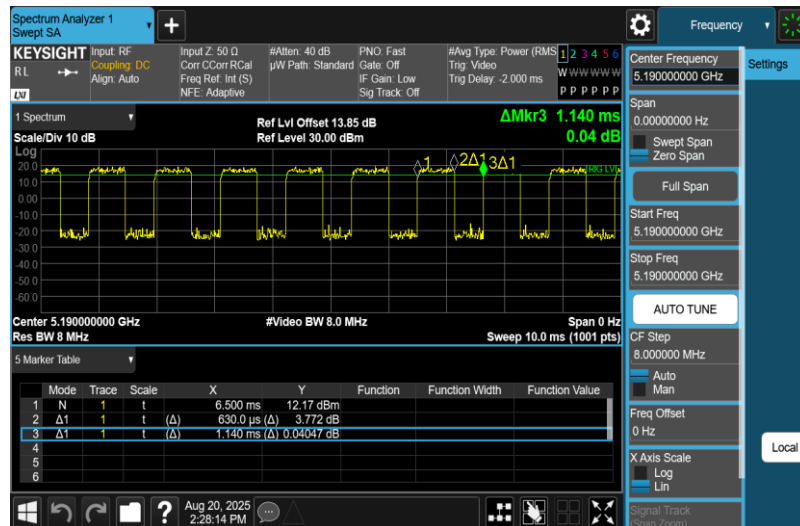
NTNV-11N40MIMO-Ant2-5190
