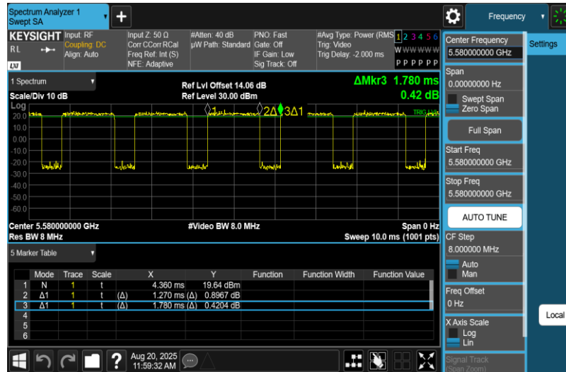
NTNV-11N20MIMO-Ant2-5580
