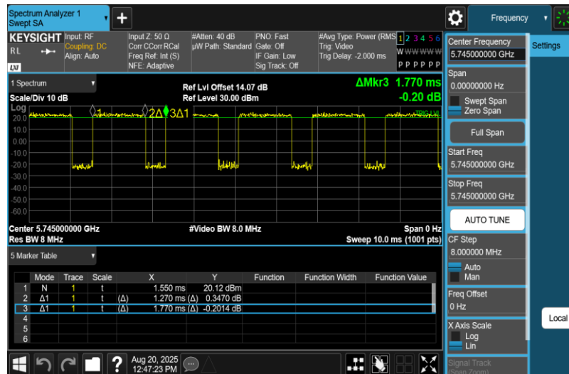
NTNV-11N20MIMO-Ant2-5745
