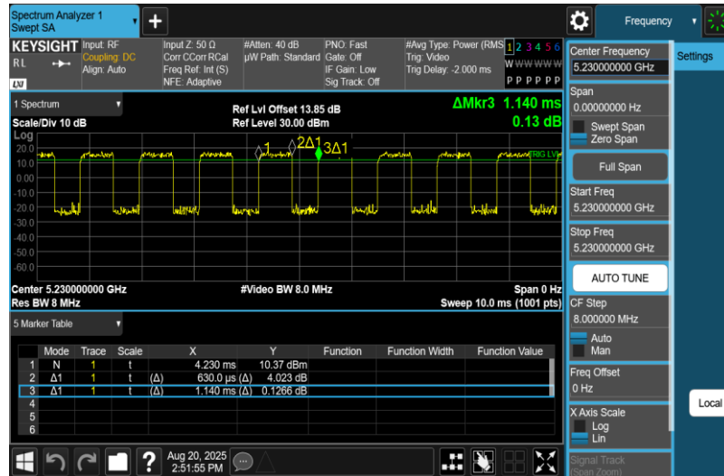
NTNV-11N40MIMO-Ant2-5230
