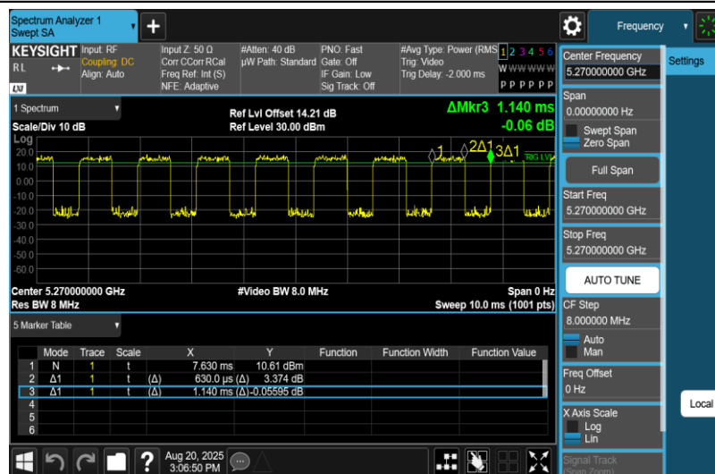
NTNV-11N40MIMO-Ant2-5270
