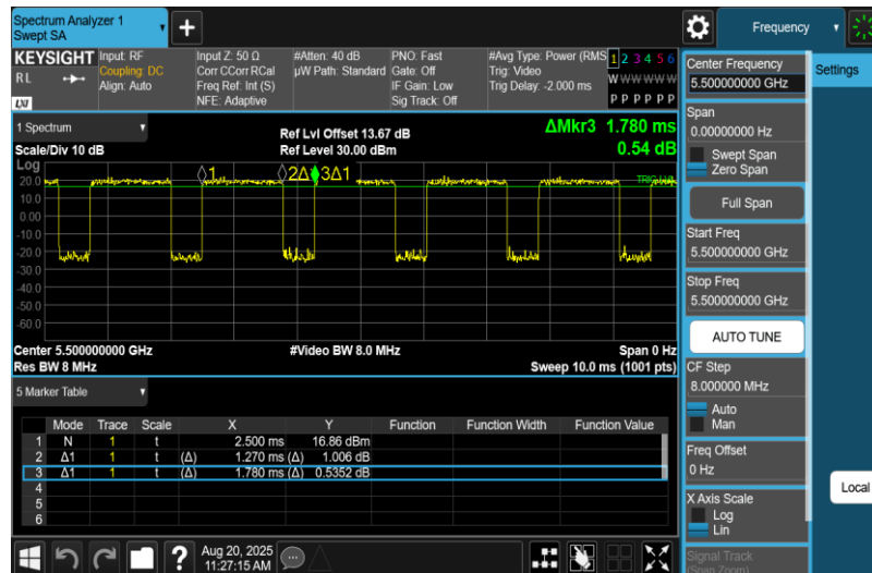
NTNV-11N20MIMO-Ant2-5500
