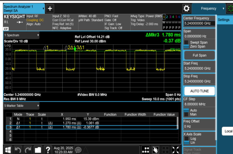
NTNV-11N20MIMO-Ant2-5240
