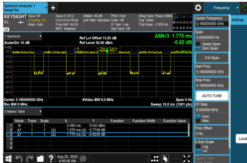
NTNV-11N20MIMO-Ant2-5180
