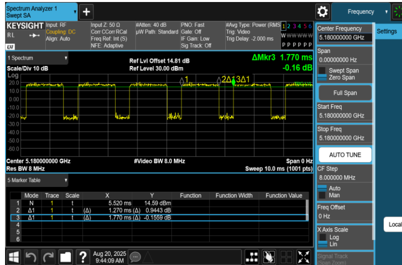
NTNV-11N20MIMO-Ant1-5180
