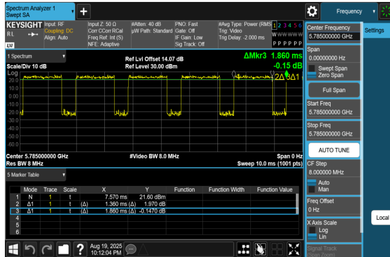
NTNV-11A-Ant2-5785
