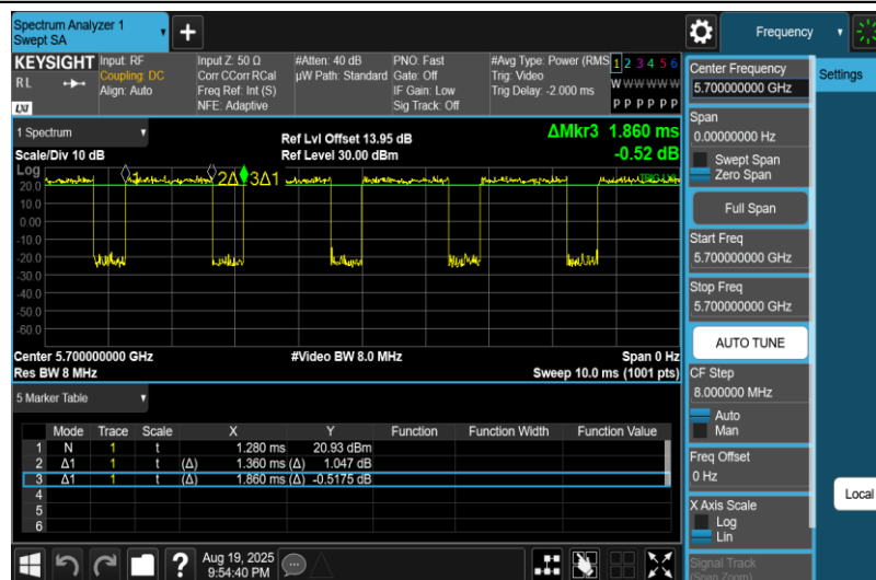
NTNV-11A-Ant2-5700
