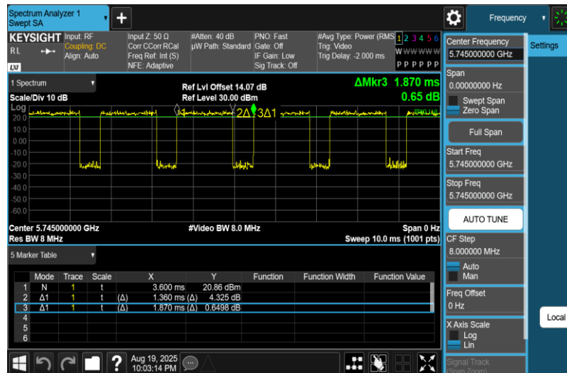
NTNV-11A-Ant2-5745
