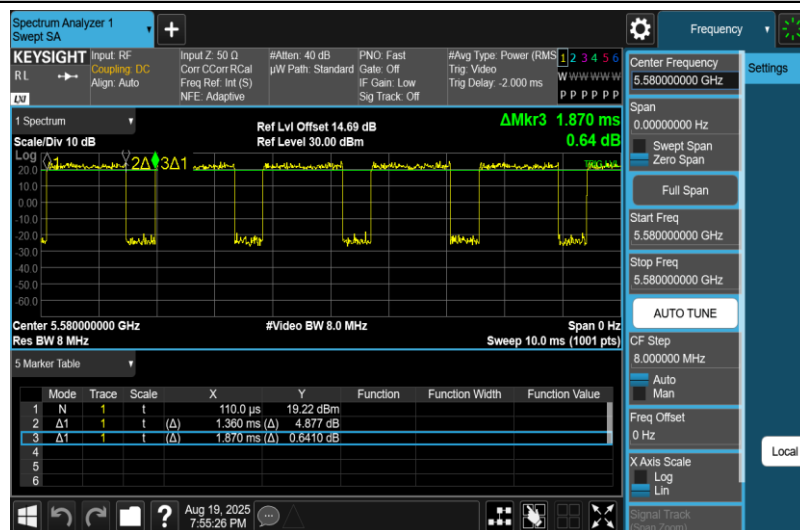
NTNV-11A-Ant1-5580
