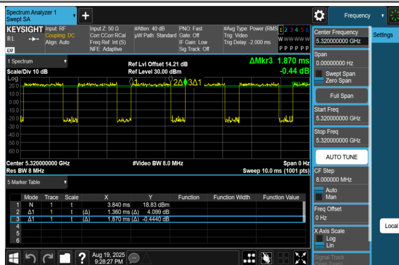
NTNV-11A-Ant2-5320
