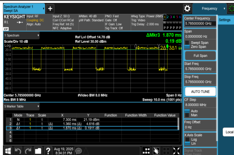
NTNV-11A-Ant1-5785
