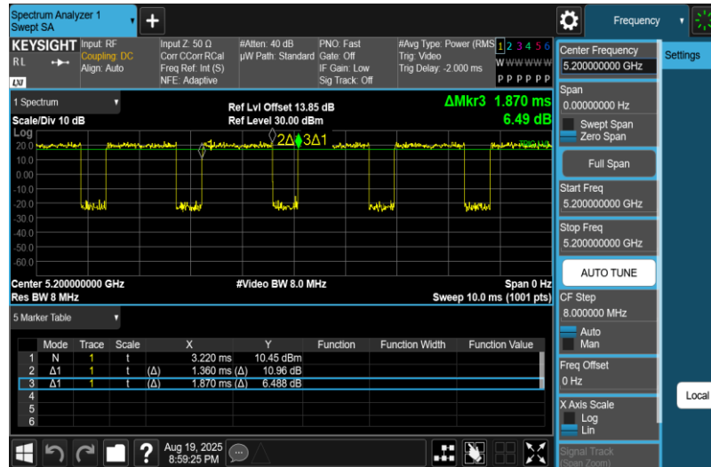
NTNV-11A-Ant2-5200
