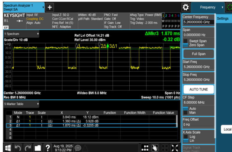
NTNV-11A-Ant2-5260
