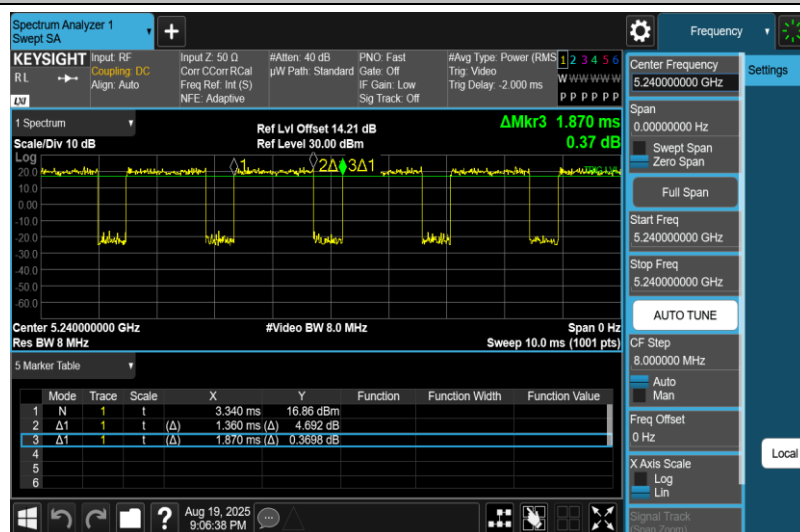
NTNV-11A-Ant2-5240
