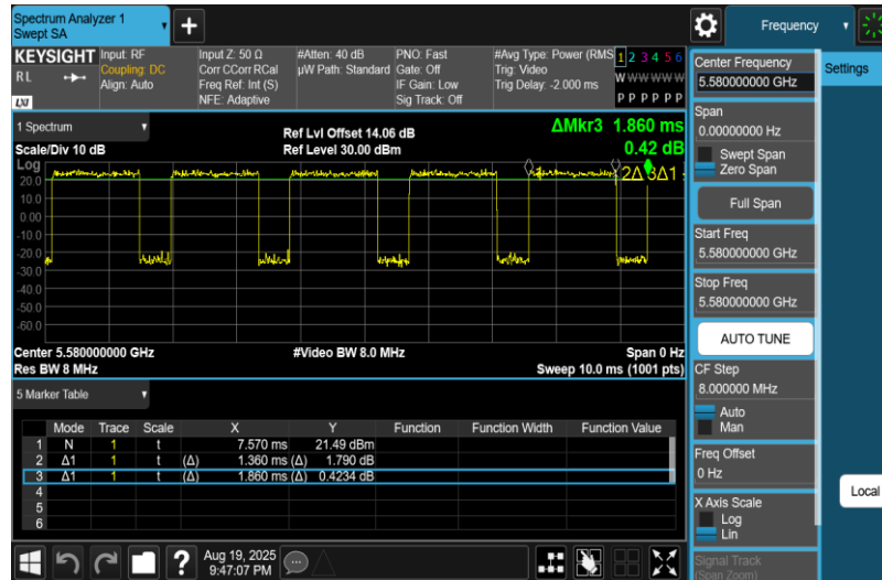
NTNV-11A-Ant2-5580
