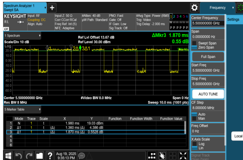
NTNV-11A-Ant2-5500
