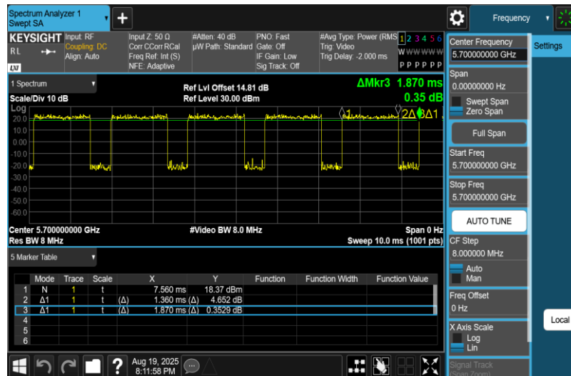
NTNV-11A-Ant1-5700
