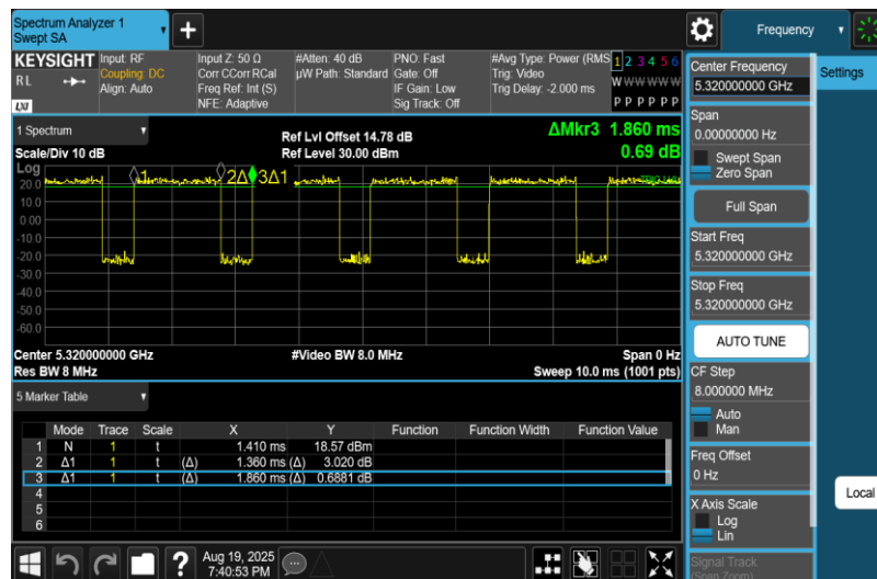
NTNV-11A-Ant1-5320
