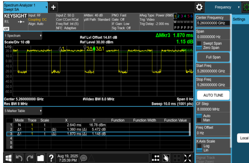
NTNV-11A-Ant1-5260
