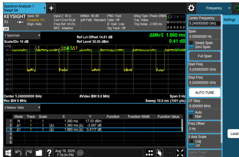
NTNV-11A-Ant1-5240
