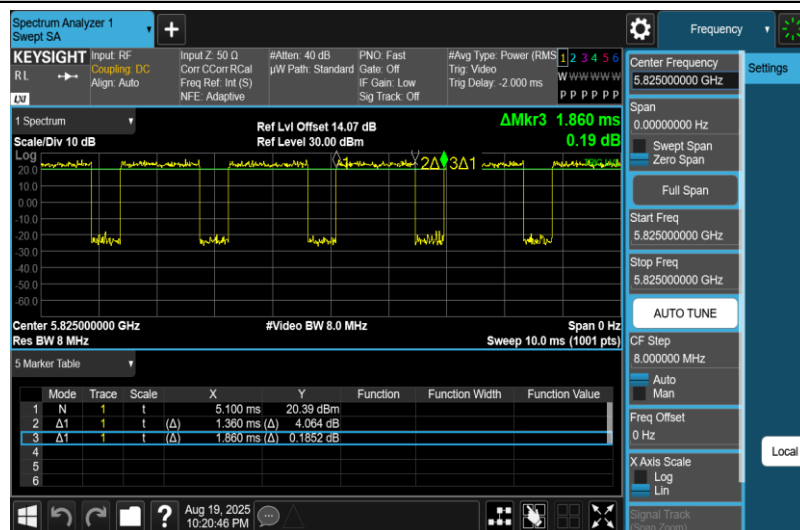
NTNV-11A-Ant2-5825
