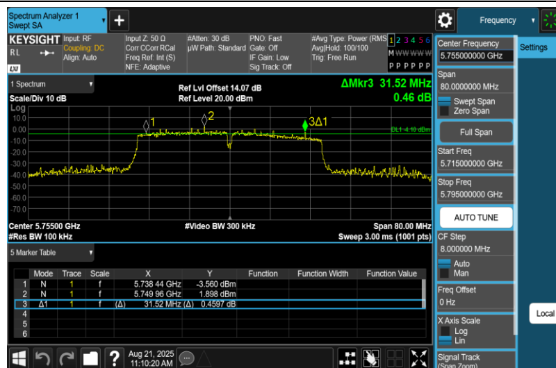
11AC40MIMO-Ant2-5755-PASS
