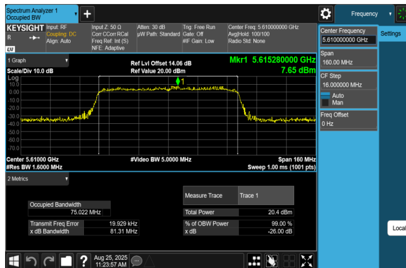
11AC80MIMO-Ant2-5610
