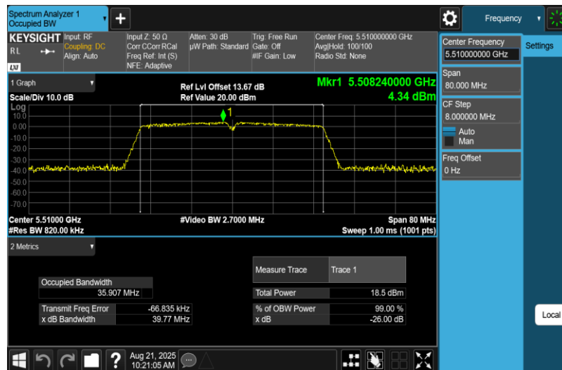
11AC40MIMO-Ant2-5510
