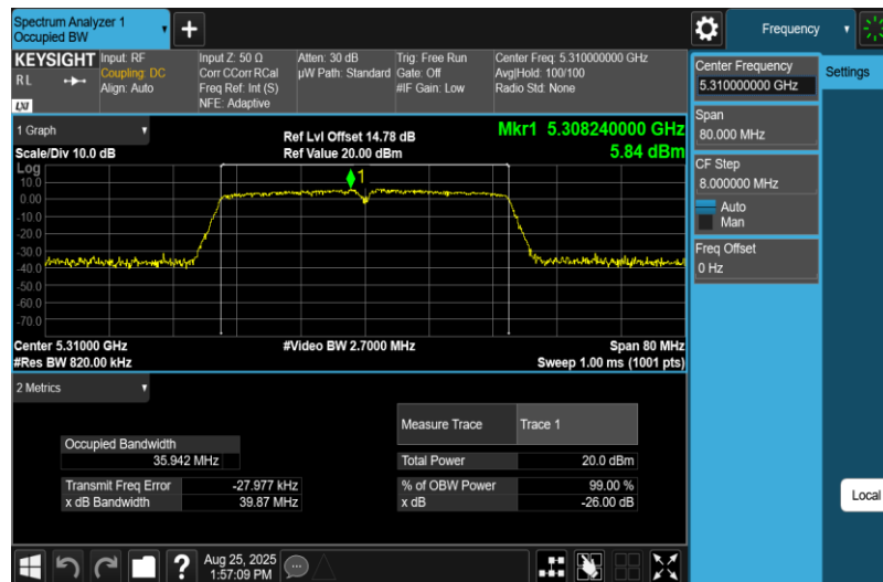
11AC40MIMO-Ant1-5310
