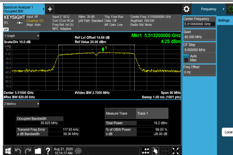
11AC40MIMO-Ant1-5510
