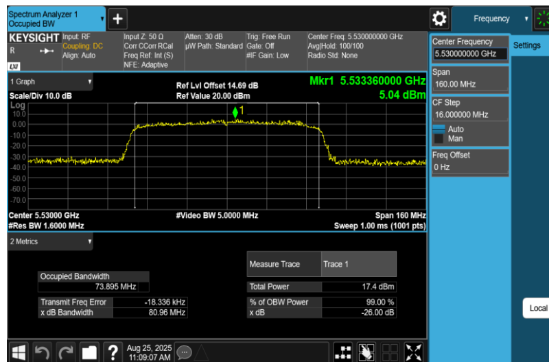
11AC80MIMO-Ant1-5530
