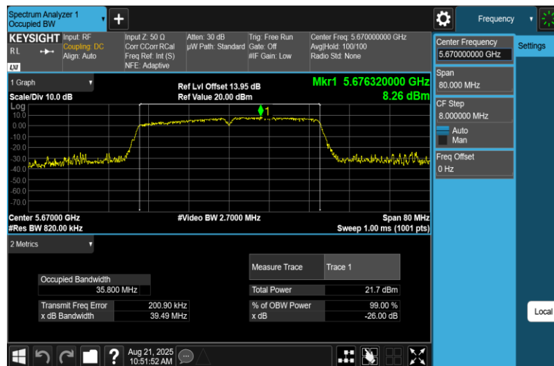
11AC40MIMO-Ant2-5670
