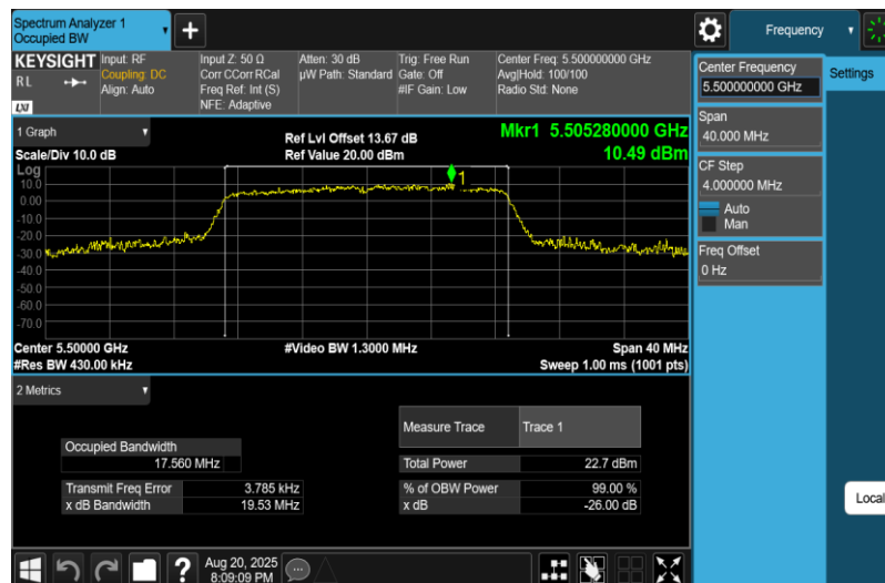
11AC20MIMO-Ant2-5500
