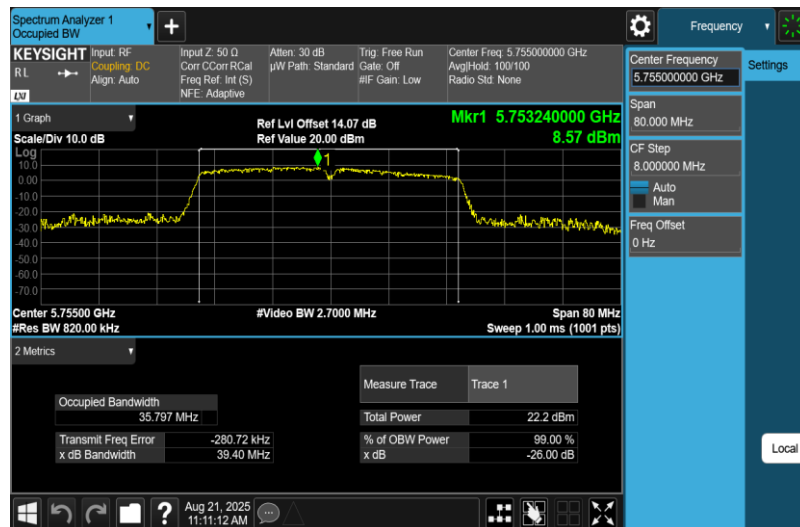
11AC40MIMO-Ant2-5755
