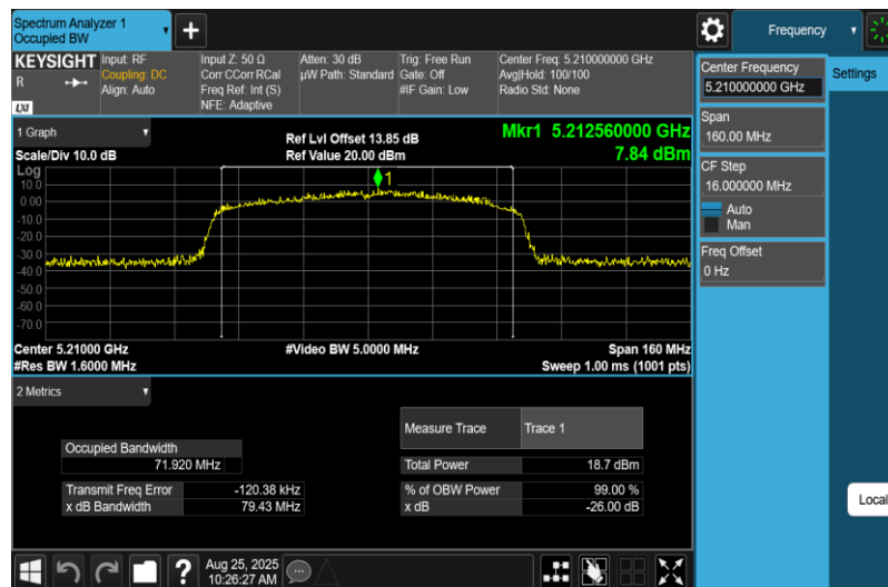
11AC80MIMO-Ant2-5210
