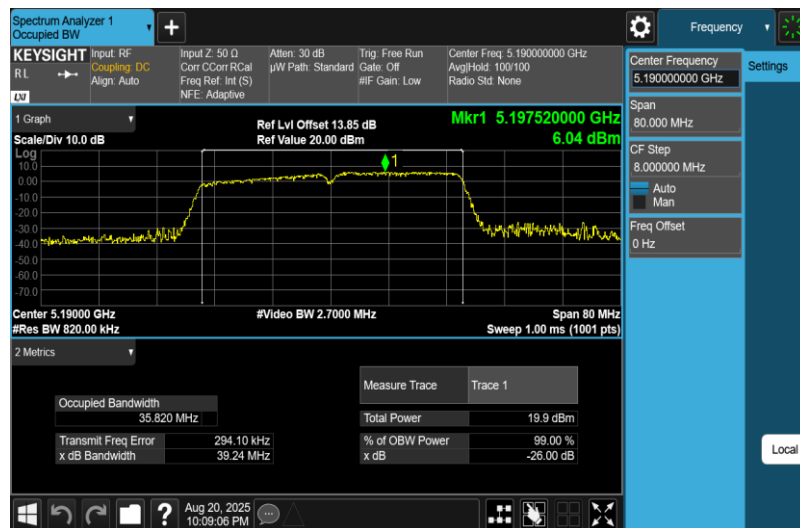
11AC40MIMO-Ant2-5190
