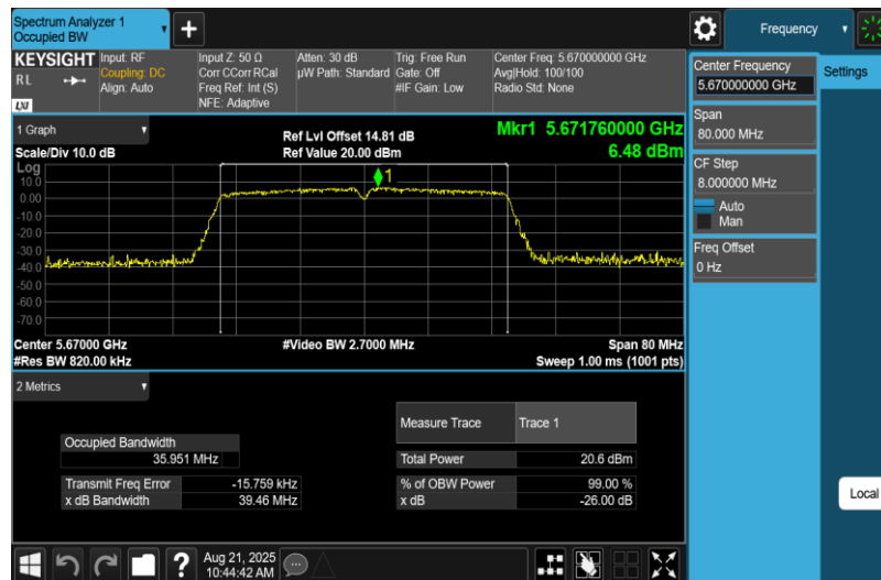
11AC40MIMO-Ant1-5670
