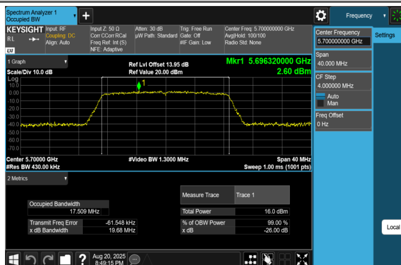
11AC20MIMO-Ant2-5700
