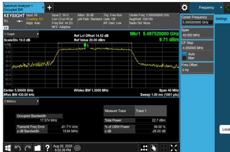
11AC20MIMO-Ant1-5500
