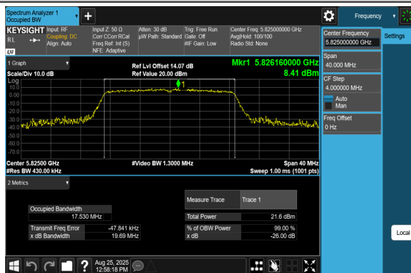
11AC20MIMO-Ant2-5825
