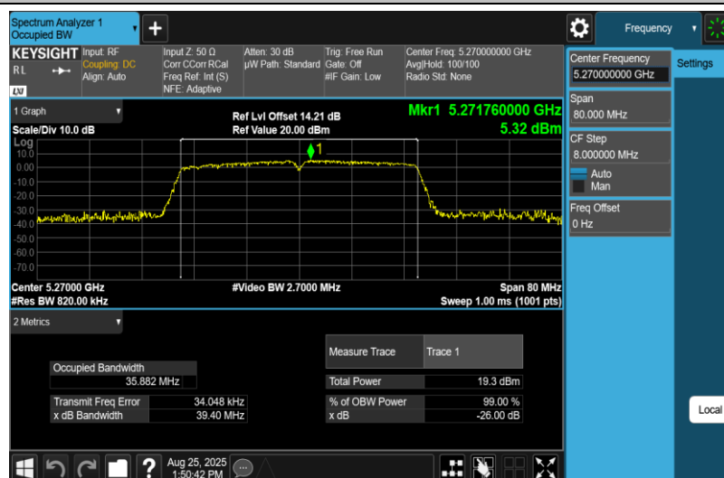
11AC40MIMO-Ant2-5270
