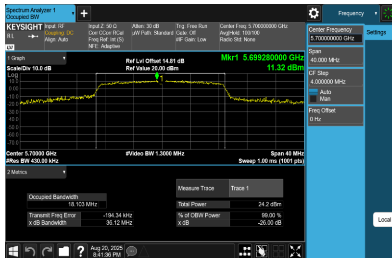
11AC20MIMO-Ant1-5700
