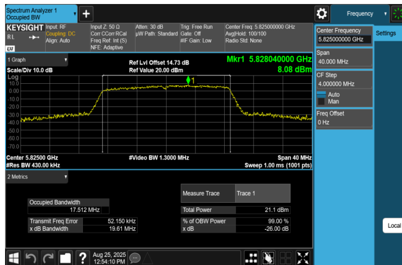
11AC20MIMO-Ant1-5825
