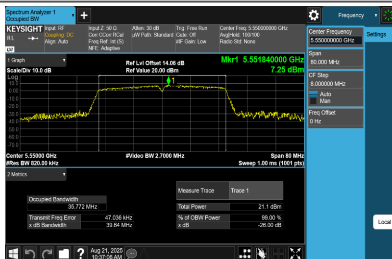
11AC40MIMO-Ant2-5550
