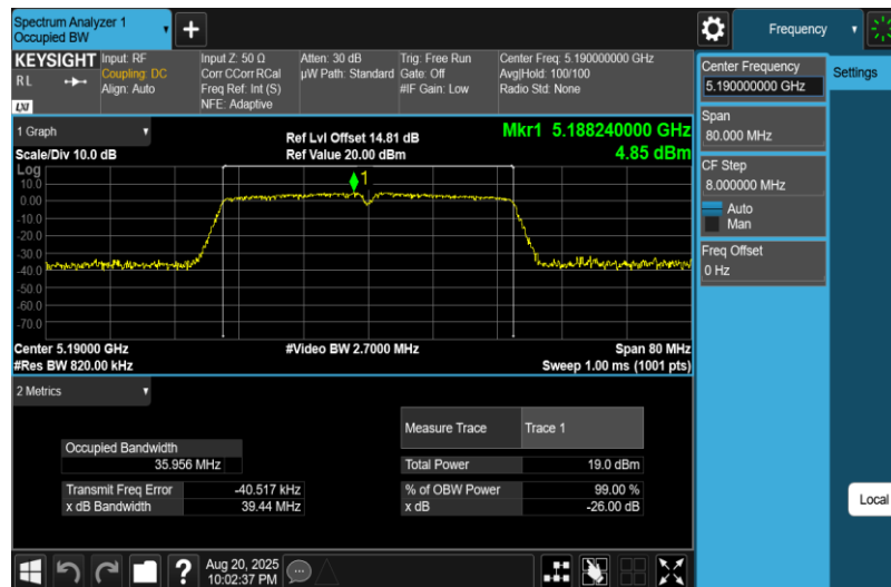
11AC40MIMO-Ant1-5190
