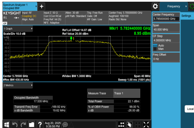
11AC20MIMO-Ant2-5785
