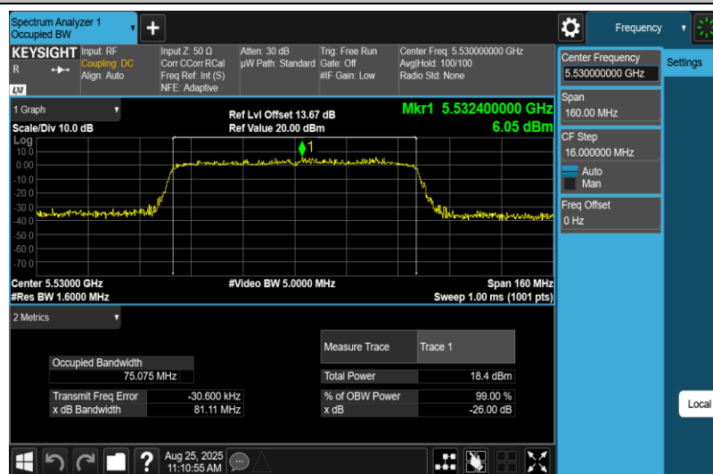
11AC80MIMO-Ant2-5530
