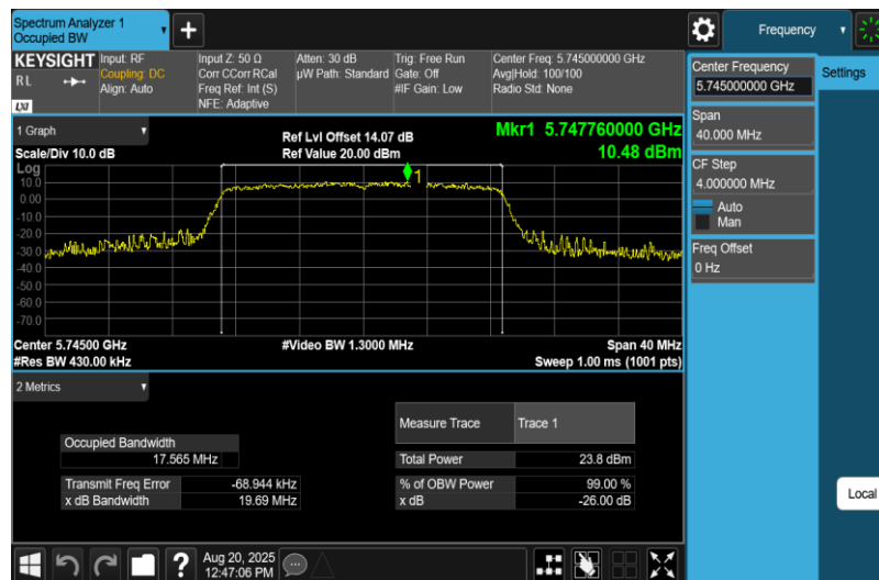
11N20MIMO-Ant2-5745
