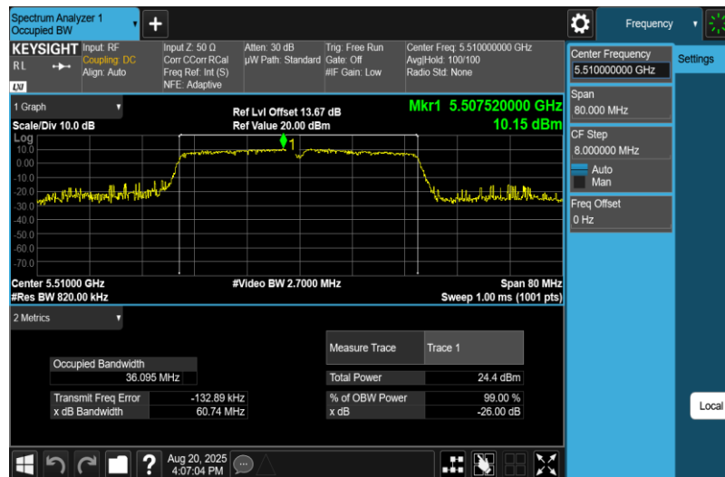
11N40MIMO-Ant2-5510
