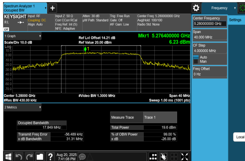
11AC20MIMO-Ant2-5280
