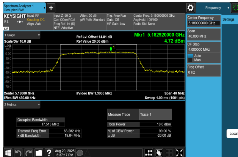
11AC20MIMO-Ant1-5180
