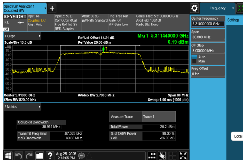
11N40MIMO-Ant2-5310
