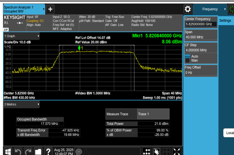
11N20MIMO-Ant2-5825
