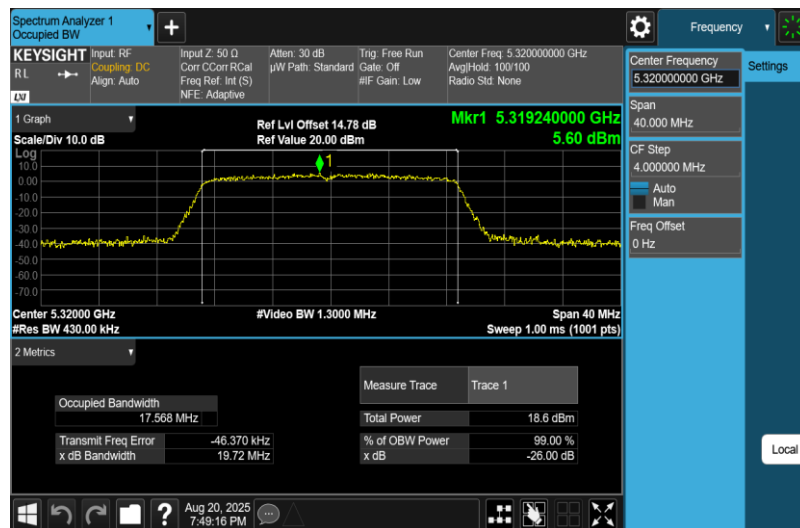
11AC20MIMO-Ant1-5320
