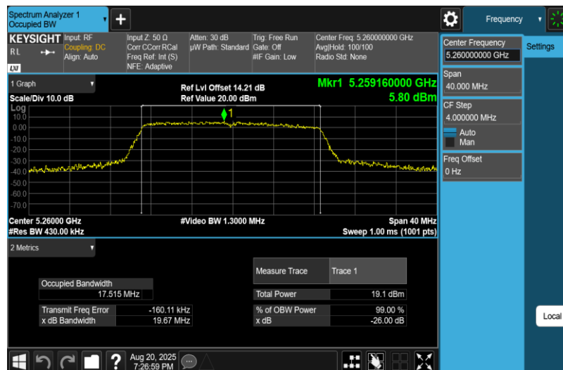
11AC20MIMO-Ant2-5260
