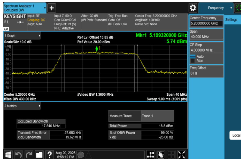
11AC20MIMO-Ant2-5200
