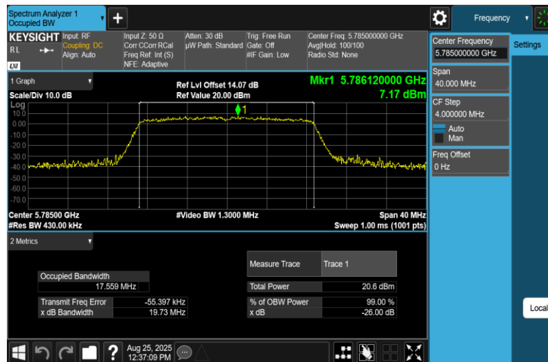
11N20MIMO-Ant2-5785
