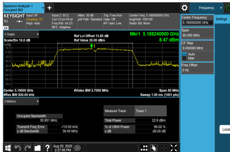
11N40MIMO-Ant2-5190
