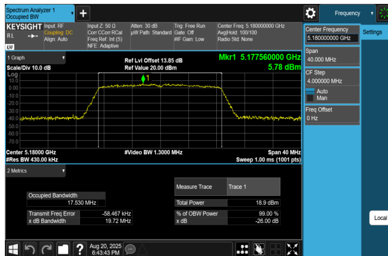
11AC20MIMO-Ant2-5180
