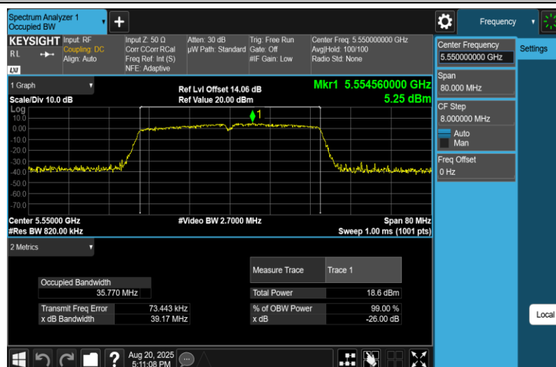
11N40MIMO-Ant2-5550
