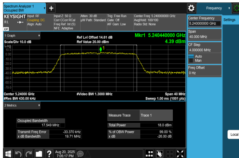
11AC20MIMO-Ant1-5240
