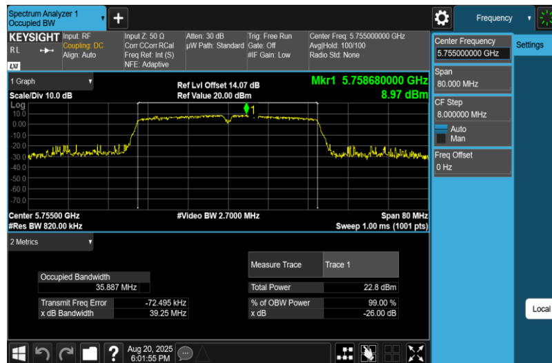
11N40MIMO-Ant2-5755
