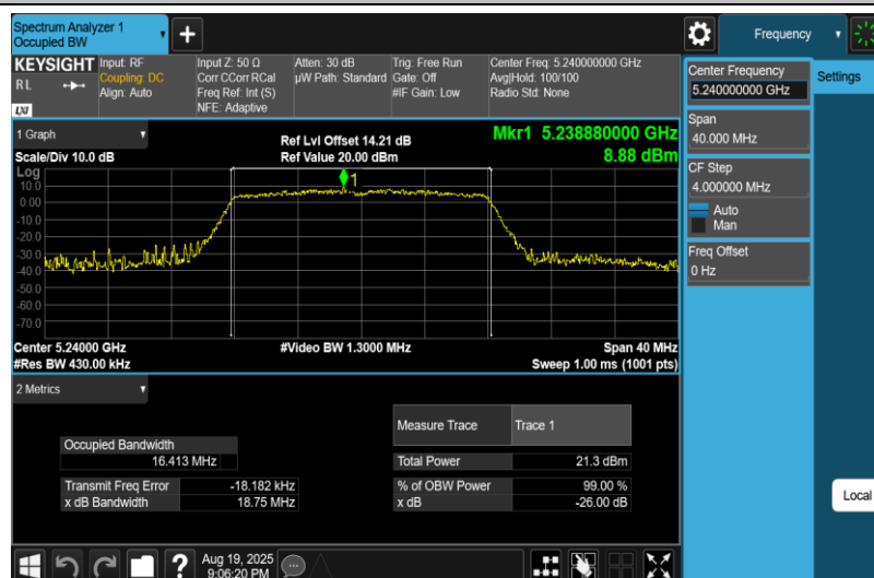
11A-Ant2-5240
