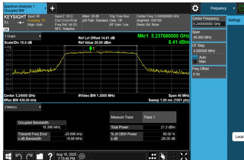
11A-Ant1-5240
