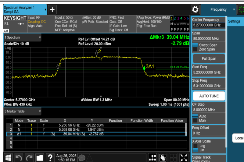
11AC40MIMO-Ant2-5270
