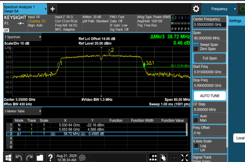
11AC40MIMO-Ant2-5550
