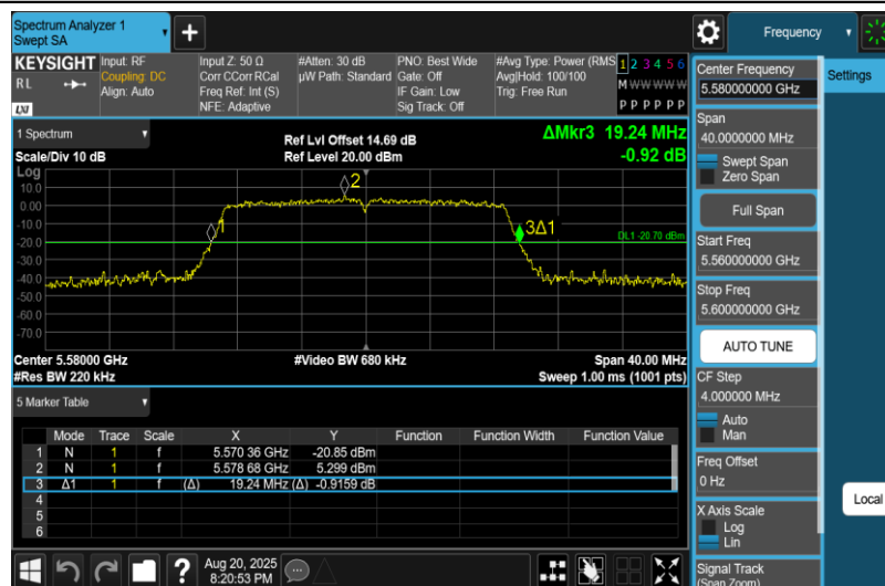
11AC20MIMO-Ant1-5580
