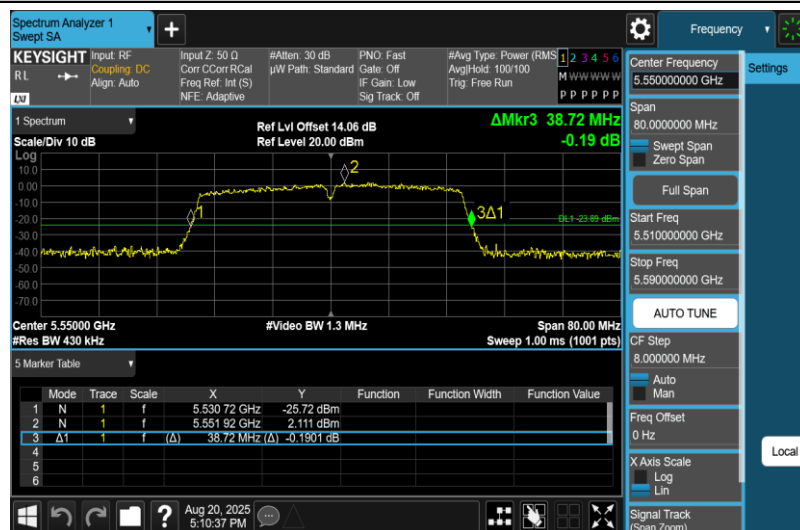
11N40MIMO-Ant2-5550
