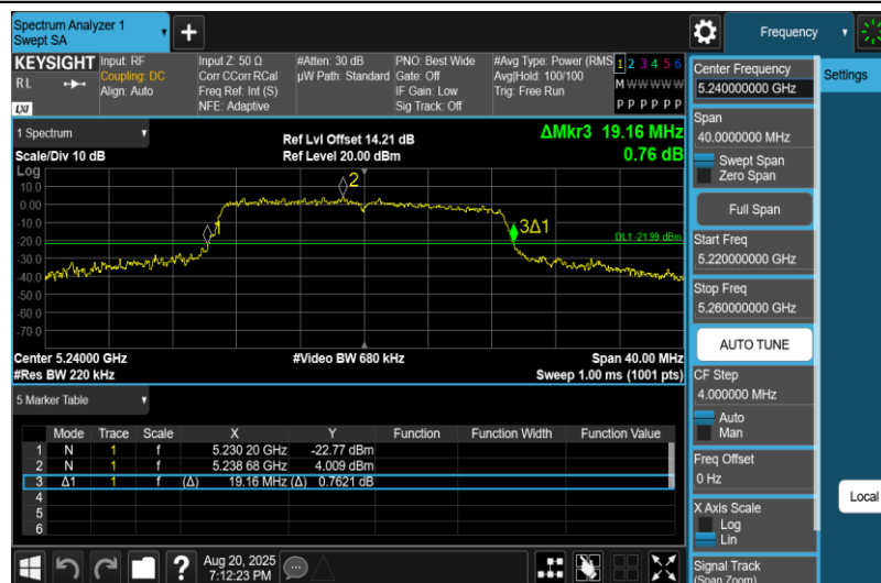
11AC20MIMO-Ant2-5240
