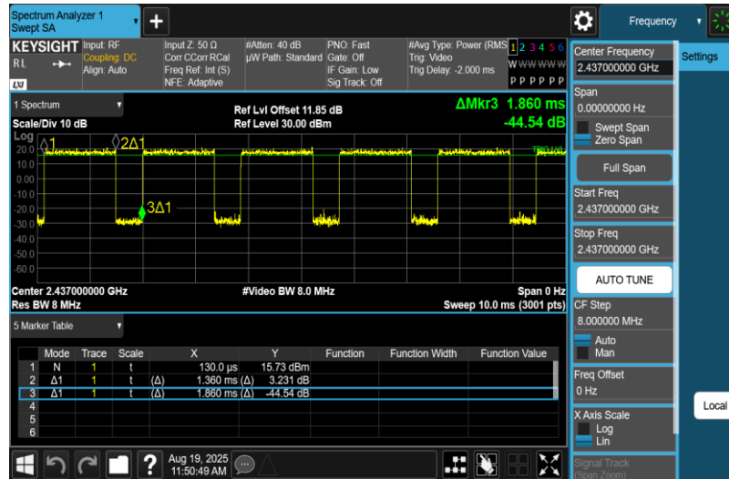
NTNV-11G-Ant2-2437
