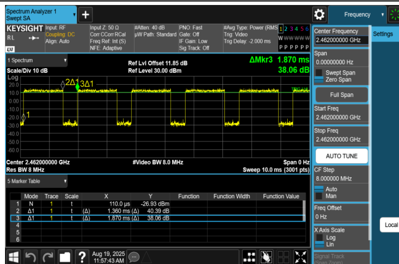
NTNV-11G-Ant2-2462
