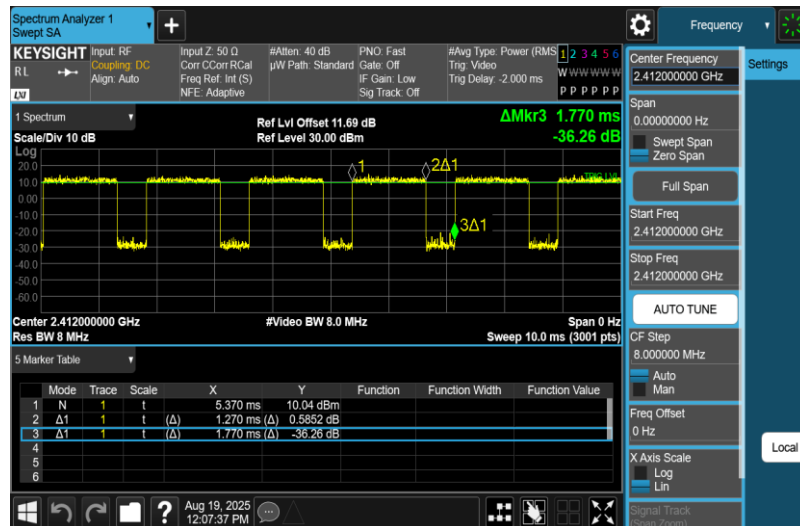
NTNV-11N20MIMO-Ant2-2412
