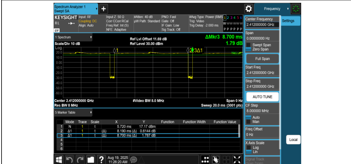
NTNV-11B-Ant2-2412
