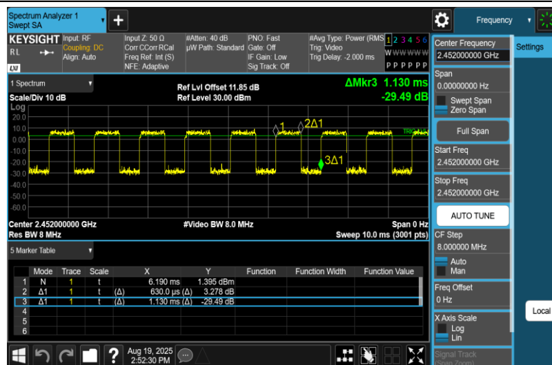
NTNV-11N40MIMO-Ant2-2452
