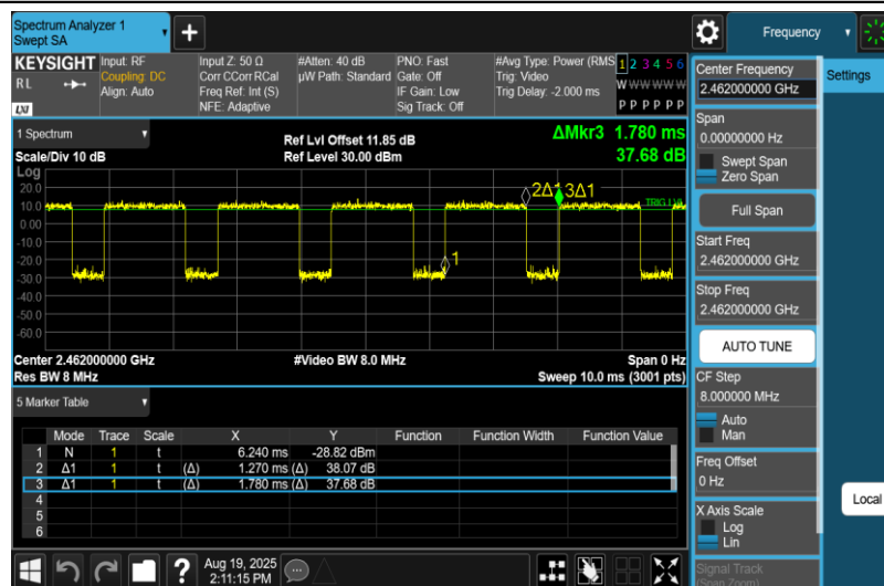
NTNV-11N20MIMO-Ant2-2462
