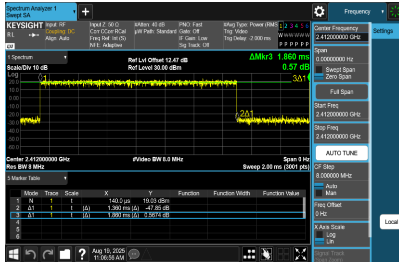
NTNV-11G-Ant1-2412
