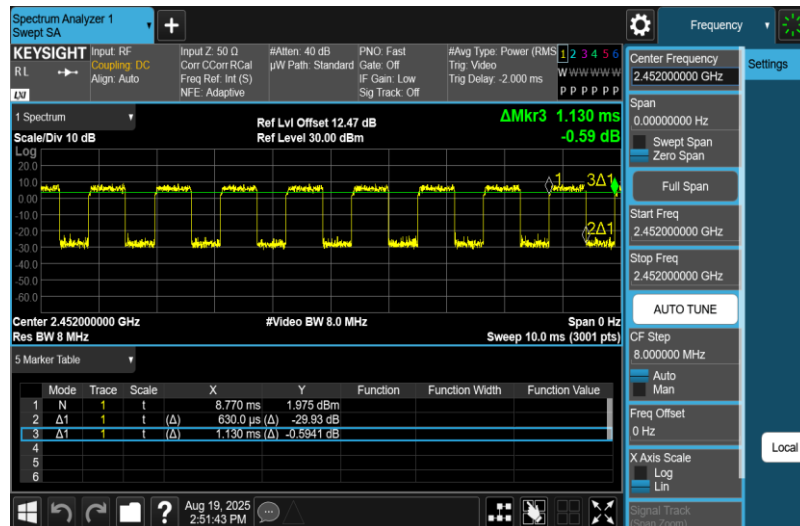
NTNV-11N40MIMO-Ant1-2452
