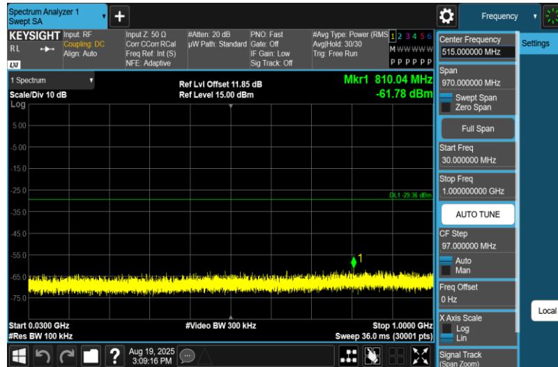
11N40MIMO-Ant2-2452-30~1000-PASS
