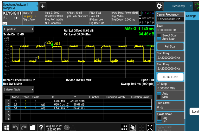
NTNV-11N40MIMO-Ant2-2422
