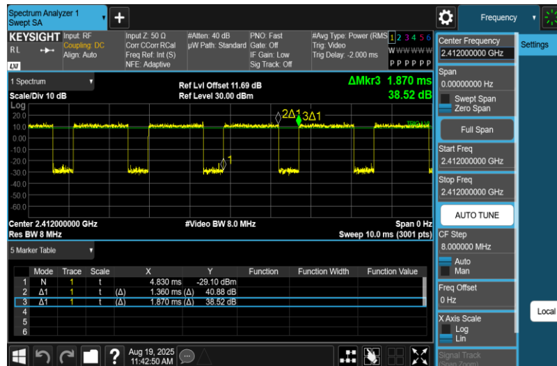
NTNV-11G-Ant2-2412
