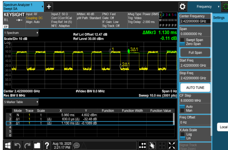
NTNV-11N40MIMO-Ant1-2422
