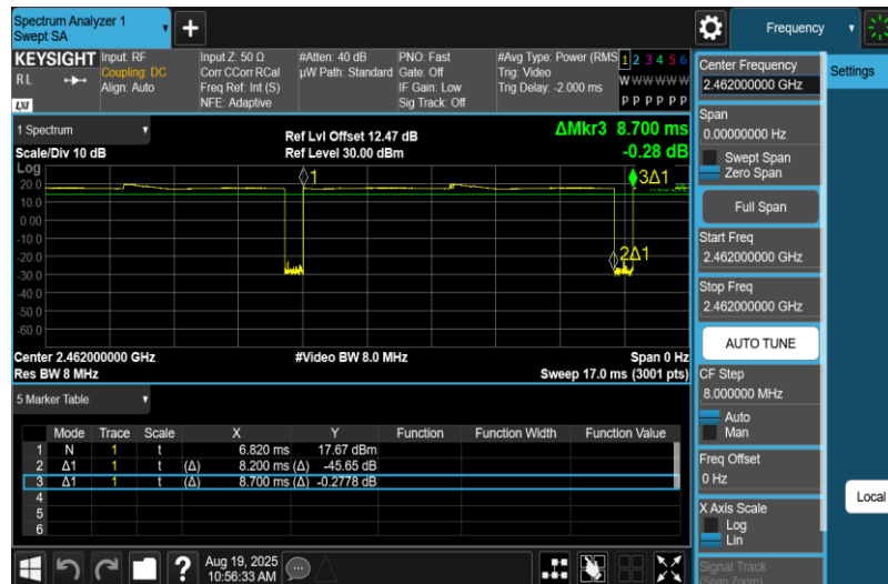
NTNV-11B-Ant1-2462
