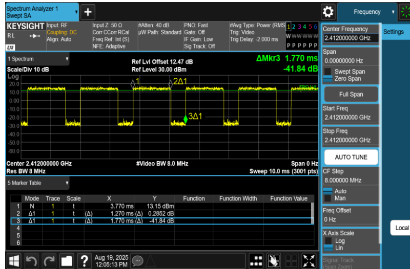
NTNV-11N20MIMO-Ant1-2412
