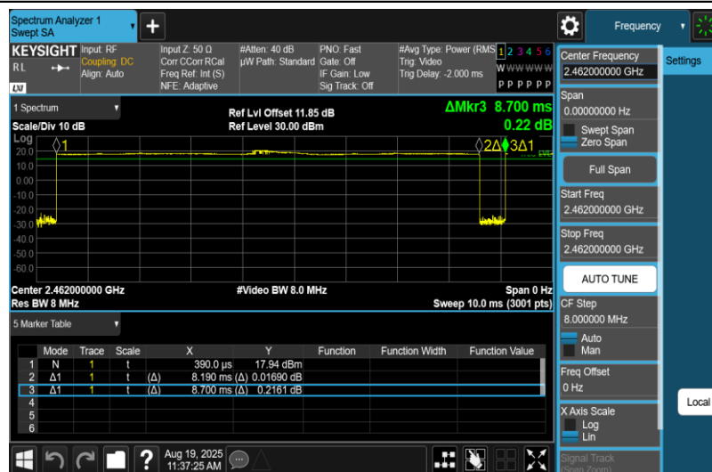
NTNV-11B-Ant2-2462
