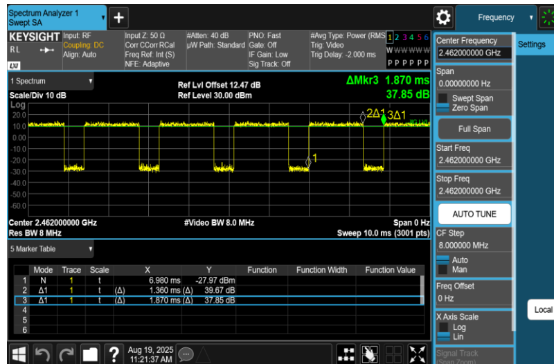
NTNV-11G-Ant1-2462
