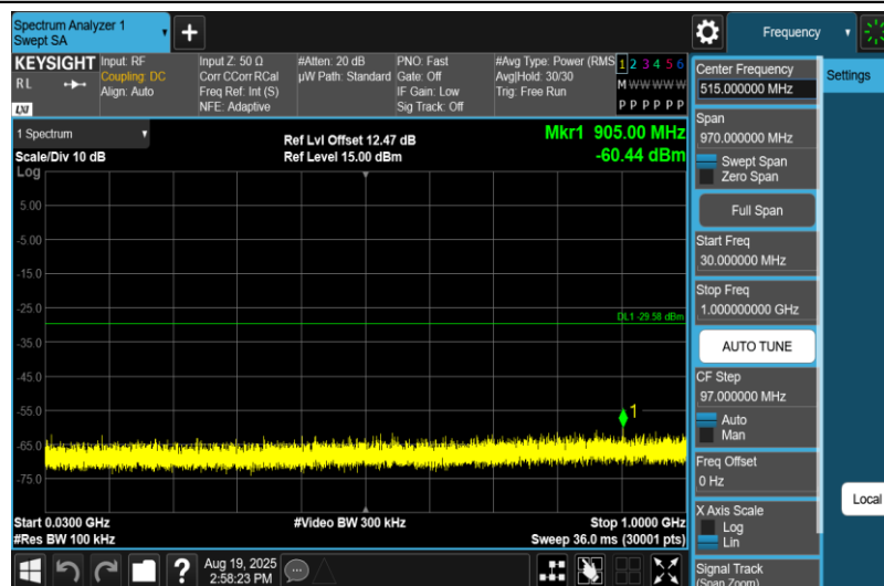
11N40MIMO-Ant1-2452-30~1000-PASS
