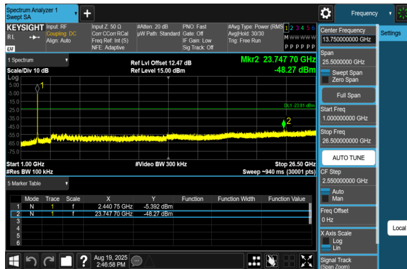
11N40MIMO-Ant1-2437-1000~26500-PASS
