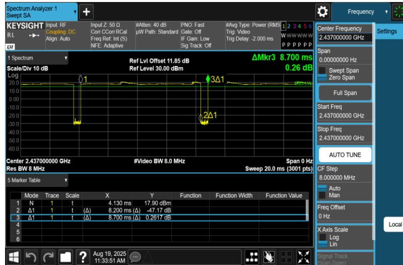
NTNV-11B-Ant2-2437
