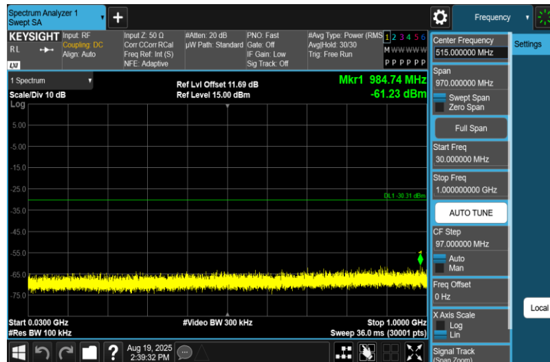
11N40MIMO-Ant2-2422-30~1000-PASS
