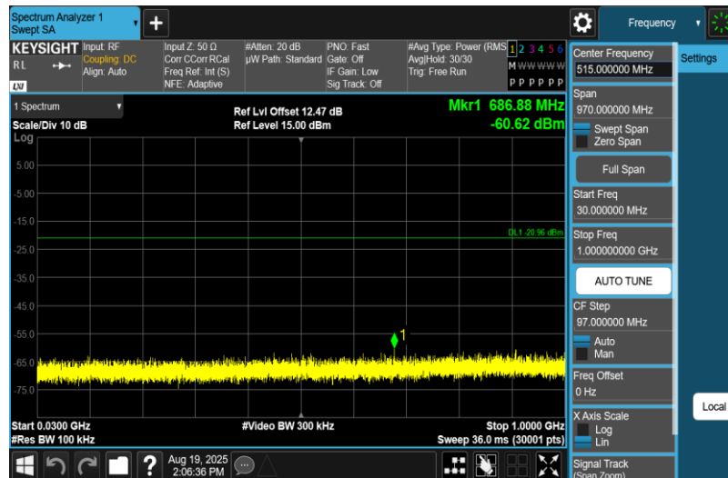
11N20MIMO-Ant1-2437-30~1000-PASS
