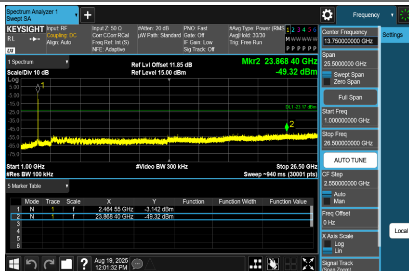
11G-Ant2-2462-1000~26500-PASS
