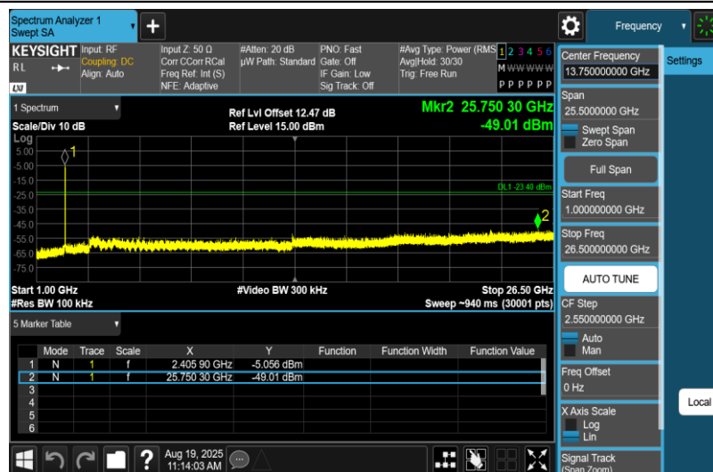
11G-Ant1-2412-1000~26500-PASS
