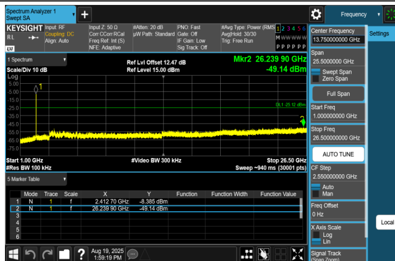
11N20MIMO-Ant1-2412-1000~26500-PASS
