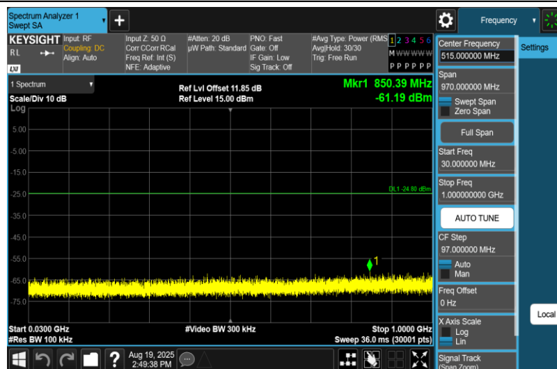
11N40MIMO-Ant2-2437-30~1000-PASS
