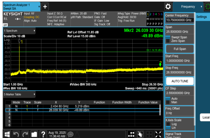
11B-Ant2-2437-1000~26500-PASS
