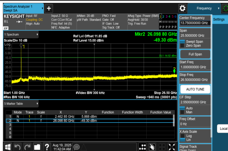
11B-Ant2-2462-1000~26500-PASS
