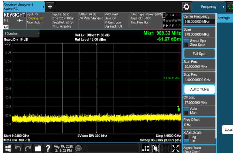
11N20MIMO-Ant2-2462-30~1000-PASS
