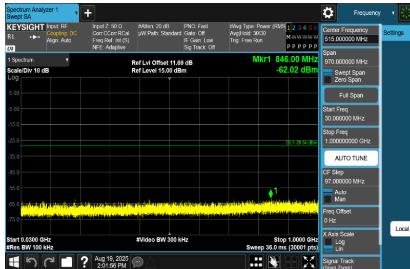
11N20MIMO-Ant2-2412-30~1000-PASS
