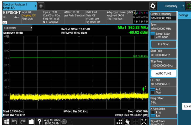
11B-Ant1-2437-30~1000-PASS
