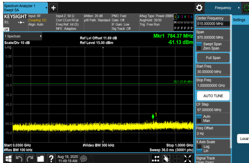
11G-Ant2-2412-30~1000-PASS
