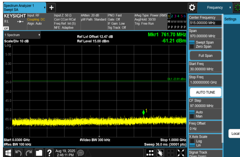
11N40MIMO-Ant1-2437-30~1000-PASS
