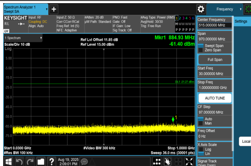
11N20MIMO-Ant2-2437-30~1000-PASS
