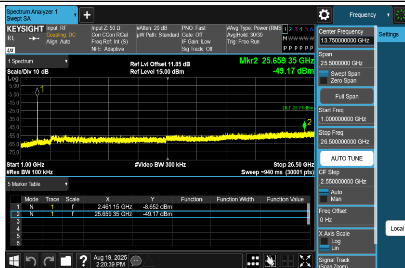
11N20MIMO-Ant2-2462-1000~26500-PASS
