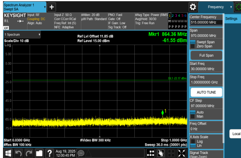
11G-Ant2-2462-30~1000-PASS
