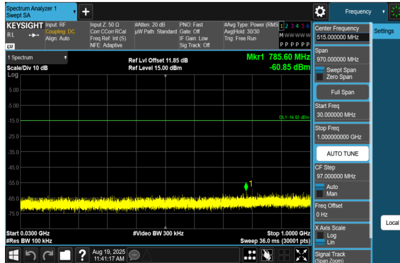
11B-Ant2-2462-30~1000-PASS
