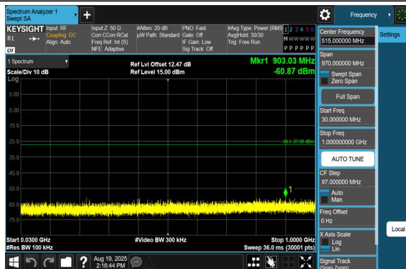
11N20MIMO-Ant1-2462-30~1000-PASS
