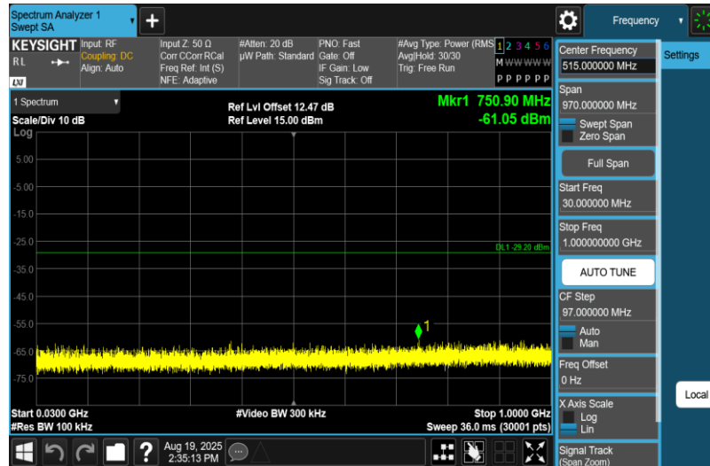
11N40MIMO-Ant1-2422-30~1000-PASS
