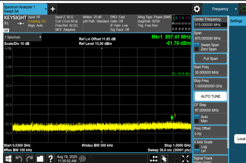
11B-Ant2-2437-30~1000-PASS
