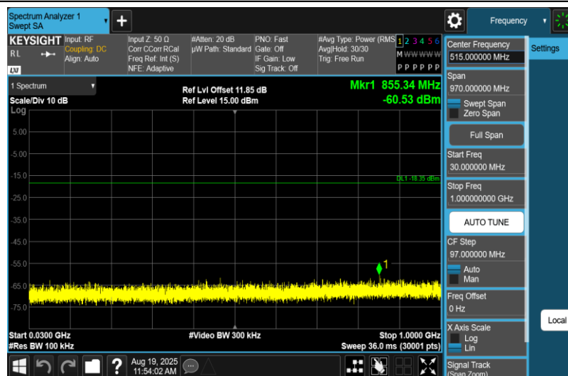
11G-Ant2-2437-30~1000-PASS
